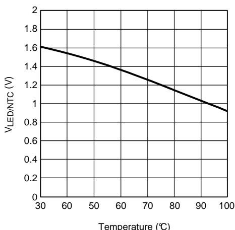
Figure 39. Thermistor Resistive Divider Response vs Temperature VLED/NTC vs Temp ( V_{BIAS} = 1.8V , THERMISTOR = 10k\Omega at +25^{\circ}C , \beta = 3380 , R_{BIAS} = 972\Omega )
