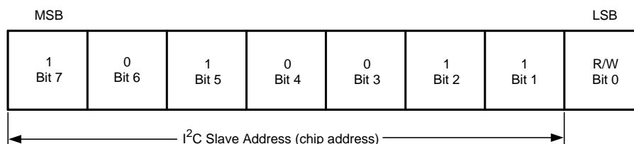
Figure 37. Device Address
