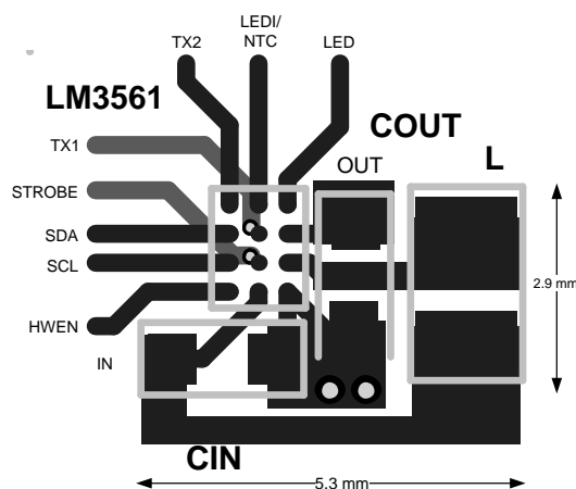
Figure 2. Example Layout
