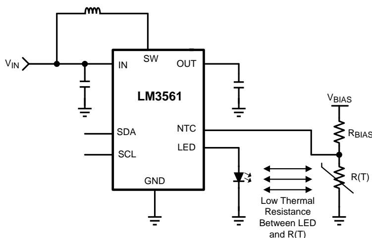
Figure 38. NTC Circuit
