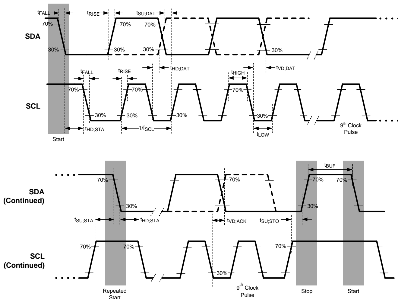
Figure 36. I²C-Compatible Timing
