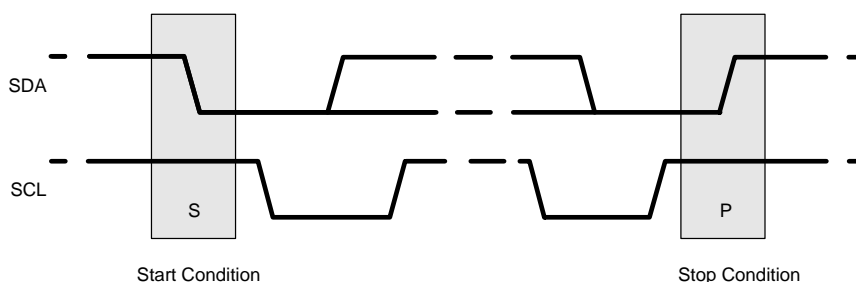
Figure 35. Start and Stop Sequences
