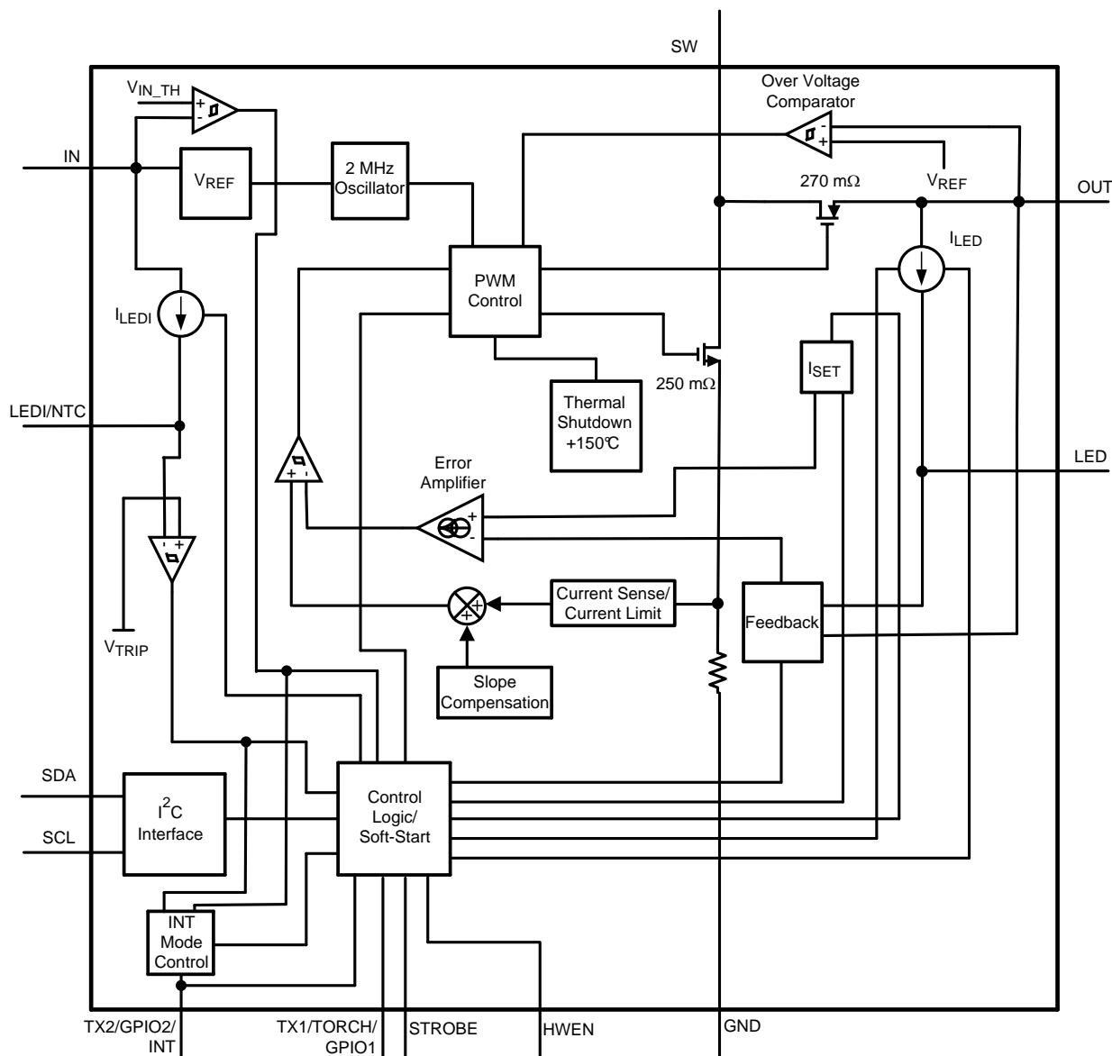
Figure 24. Block Diagram
