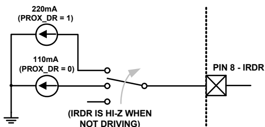
FIGURE 4. CURRENT DRIVE MODE OPTIONS
