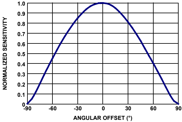
FIGURE 8. ANGULAR SENSITIVITY
