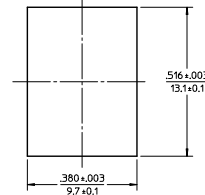
RECOMMENDED MOUNTING CUTOUT FOR .063" THICK PANEL
