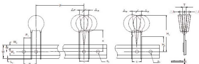
Figure 2 - PTR060V0250-PTR060V0375
