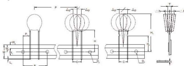
Figure 1 - PTR060V0010-PTR060V0185
