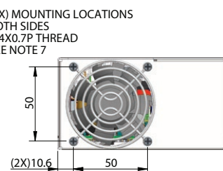
DETAIL A SCALE 1.500
