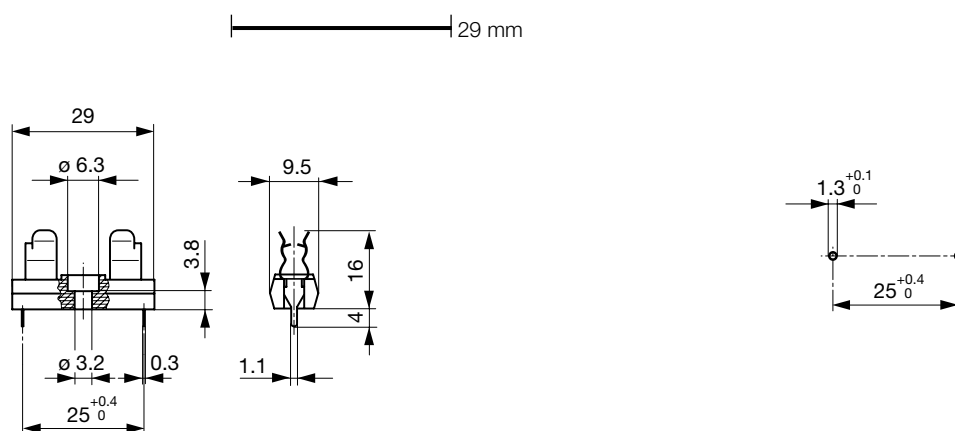
Drilling diagram
