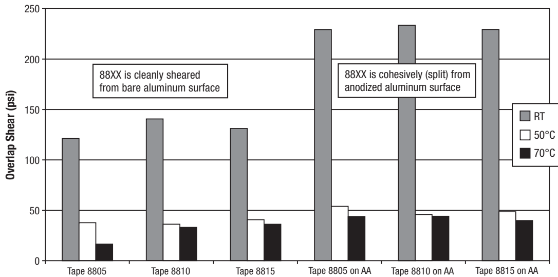
3M™ Thermally Conductive Adhesive Transfer Tapes
