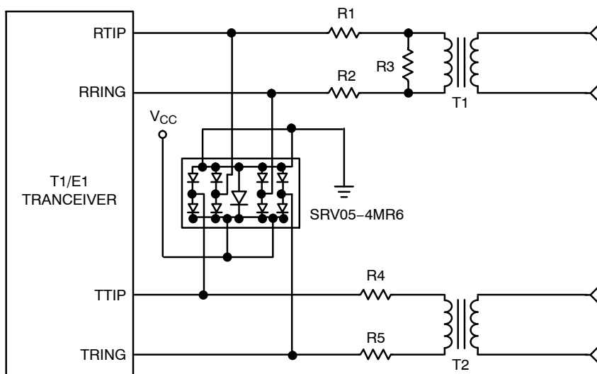
Figure 11. T1/E1 Interface Protection
