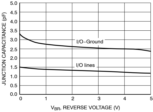
Figure 6. Junction Capacitance vs Reverse Voltage
