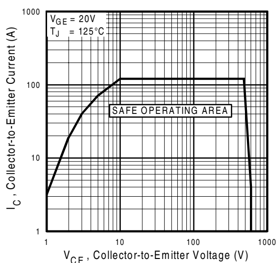
Fig. 12 - Turn-Off SOA
