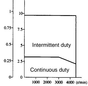
R88M-U10030LA (N·m)(kgf·cm)
