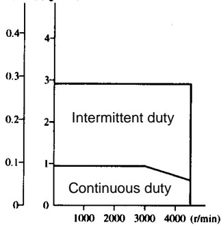
R88M-U20030LA (N·m)(kgf·cm)
