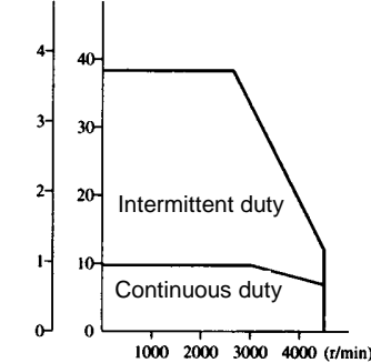
R88M-U30030LA (N·m)(kgf·cm)
