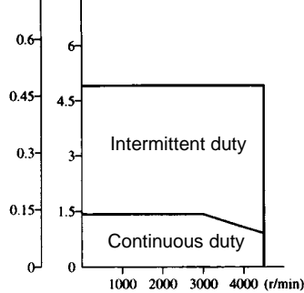
R88M-U40030HA (N·m)(kgf·cm)
