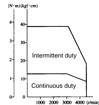
R88M-U40030HA (N·m)(kgf·cm)
