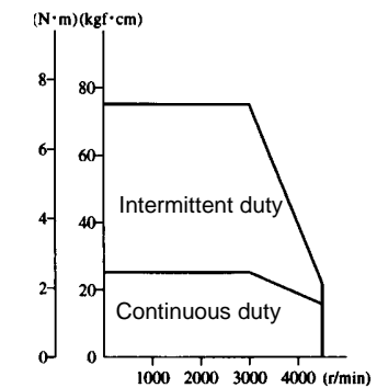
R88M-U75030HA (N·m)(kgf·cm)
