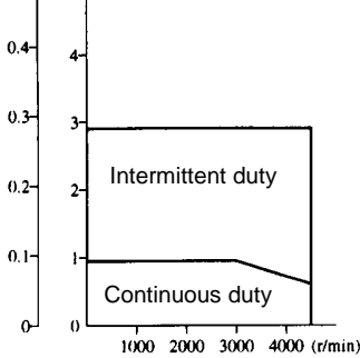
R88M-U20030HA (N·m)(kgf·cm)
