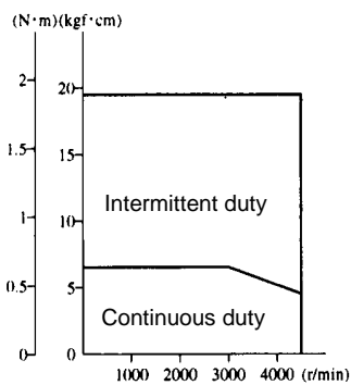
R88M-U20030HA (N·m)(kgf·cm)
