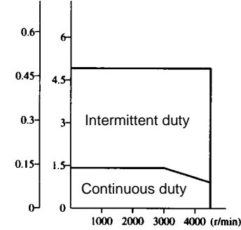
R88M-U30030LA (N·m)(kgf·cm)
