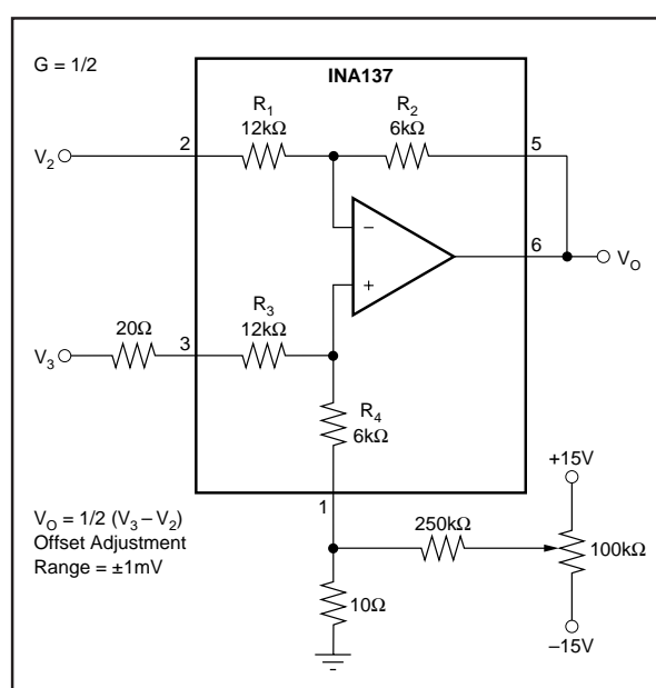
FIGURE 3. Offset Adjustment.
