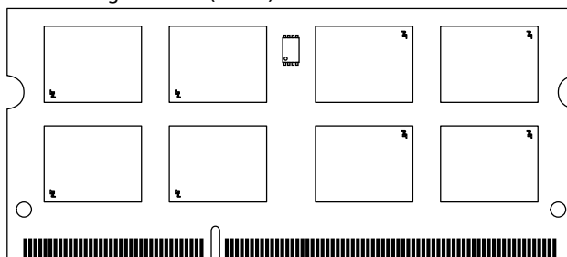
Figure 1: 204-Pin SODIMM (MO-268 R/C F)
