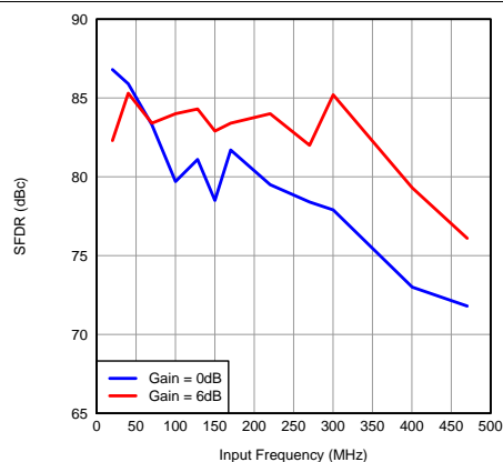
Figure 74. SFDR vs Input Frequency
