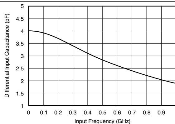
Figure 139. ADC Analog Input Capacitance ( C_{IN} ) Across Frequency
