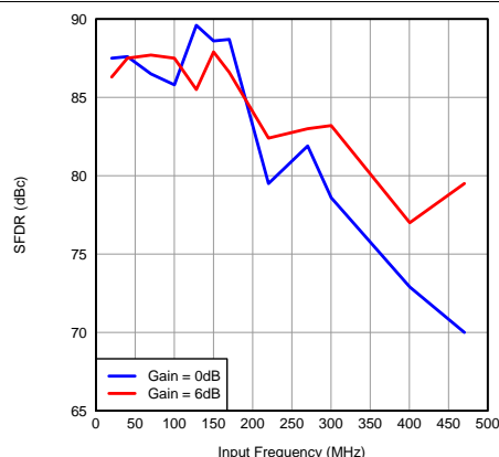
Figure 91. SFDR vs Input Frequency
