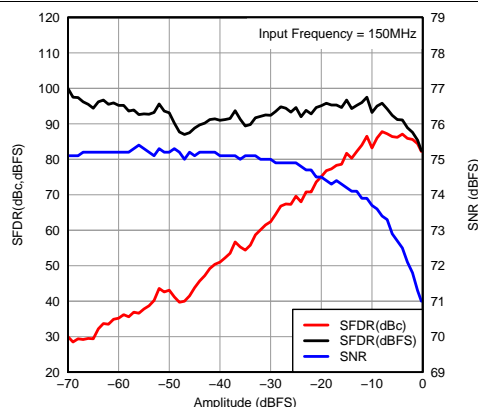
Figure 59. Performance vs Input Amplitude
