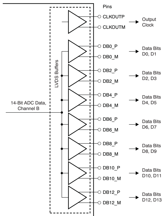
Figure 154. LVDS Interface
