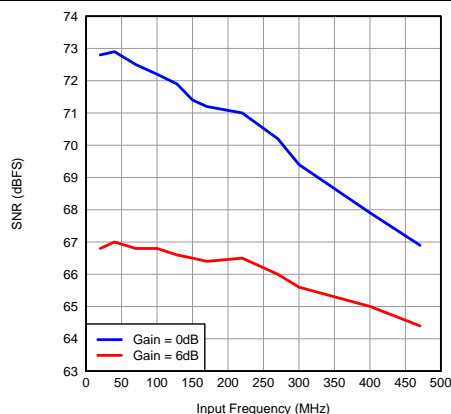
Figure 12. SNR vs Input Frequency
