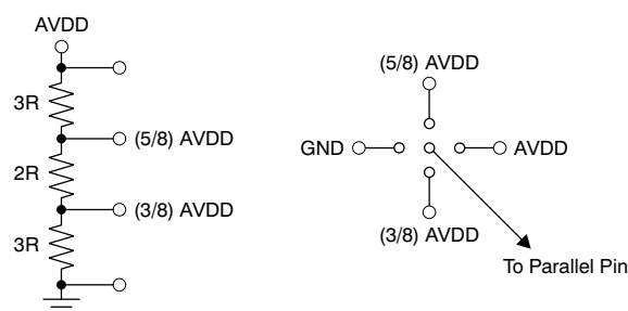
Figure 150. Simple Scheme to Configure the Parallel Pins
