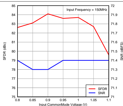
Figure 61. Performance vs Input Common-Mode Voltage
