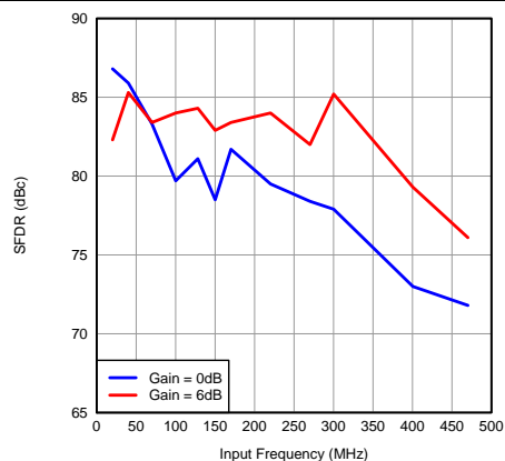
Figure 11. SFDR vs Input Frequency
