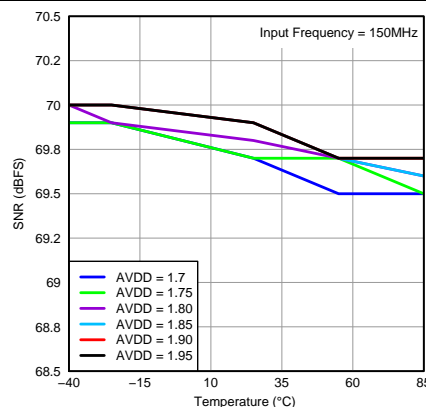
Figure 99. SNR vs Temperature and AVDD Supply
