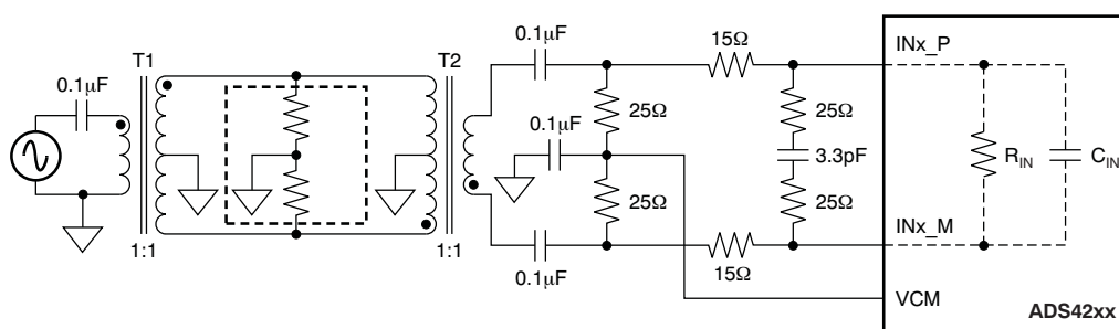
Figure 140. Drive Circuit with Low Bandwidth (for Low Input Frequencies Less Than 150 MHz)
