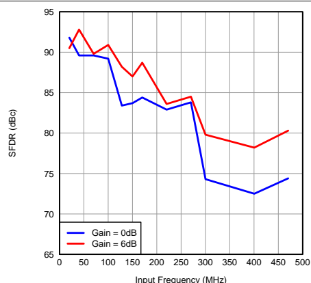
Figure 53. SFDR vs Input Frequency
