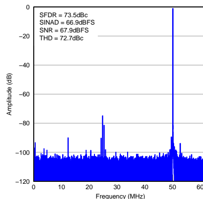
Figure 89. FFT for 300-MHz Input Signal
