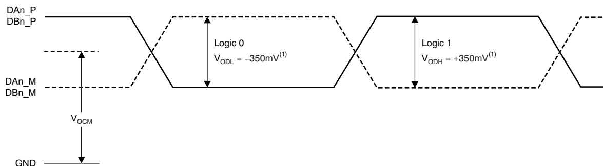
Figure 5. LVDS Output Voltage Levels
