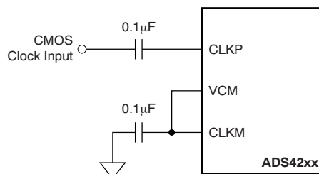
Figure 148. Single-Ended Clock Driving Circuit
