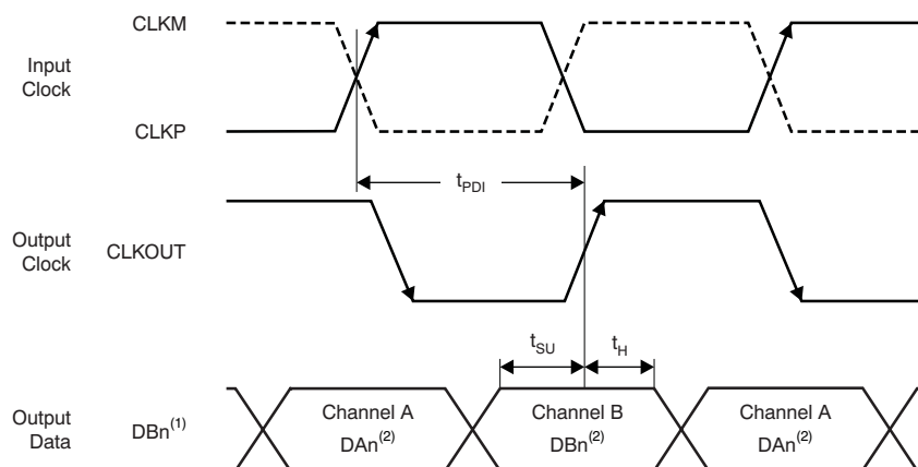
Figure 159. Multiplexed Mode Timing Diagram
