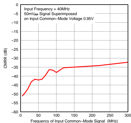
Figure 124. CMRR vs Test Signal Frequency
