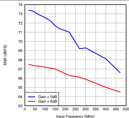
Figure 33. SNR vs Input Frequency
