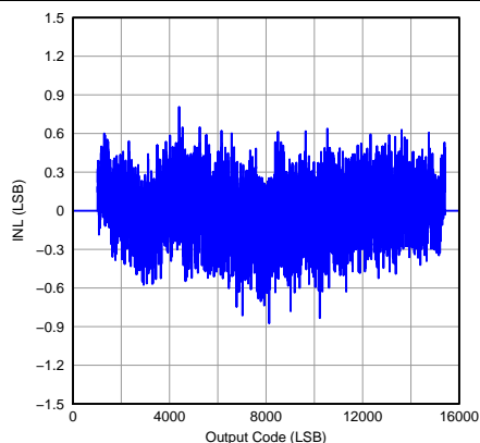
Figure 68. Integrated Nonlinearity
