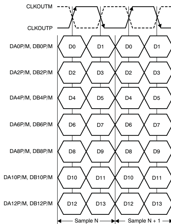
Figure 155. DDR LVDS Interface Timing
