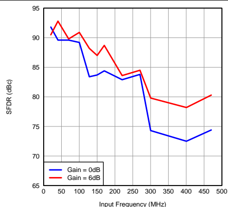
Figure 109. SFDR vs Input Frequency
