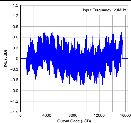
Figure 26. Integrated Nonlinearity
