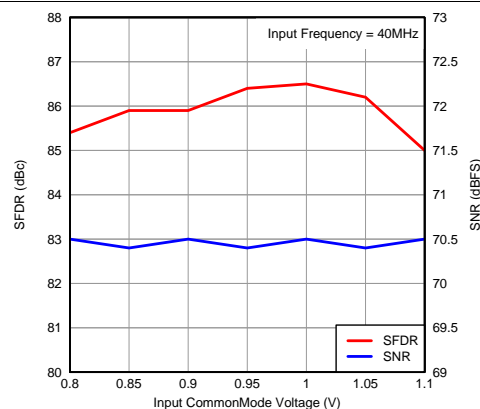
Figure 81. Performance vs Input Common-Mode Voltage
