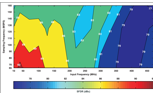
Figure 130. Spurious-Free Dynamic Range (6-dB Gain)
