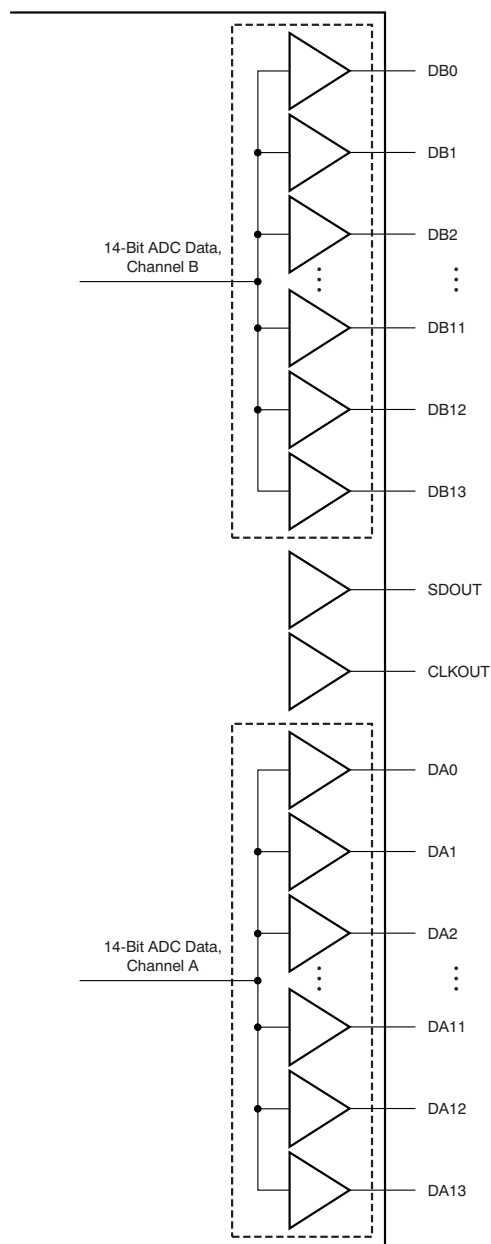
Figure 158. CMOS Outputs
