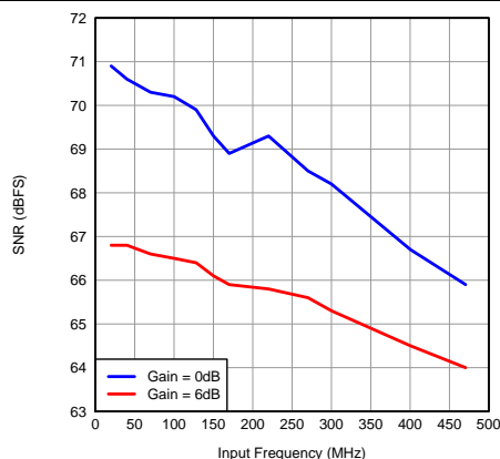
Figure 110. SNR vs Input Frequency
