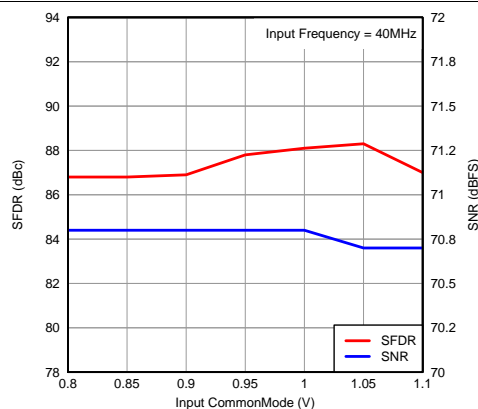
Figure 97. Performance vs Input Common-Mode Voltage
