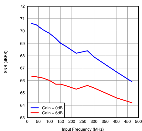
Figure 76. SNR vs Input Frequency (CMOS)
