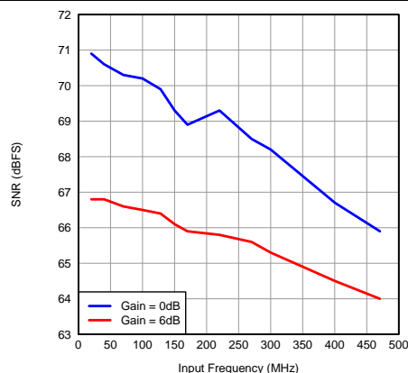
Figure 111. SNR vs Input Frequency (CMOS)
