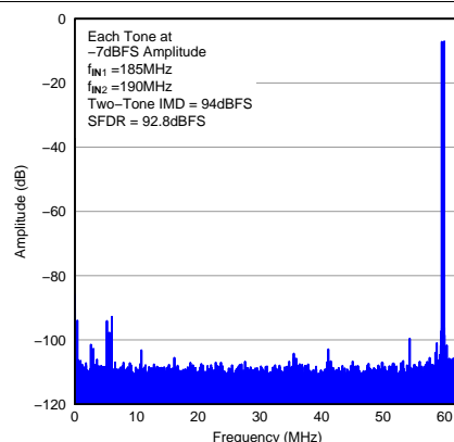
Figure 31. FFT for Two-Tone Input Signal
