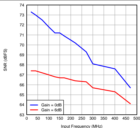
Figure 34. SNR vs Input Frequency (CMOS)
