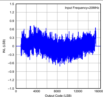
Figure 46. Integrated Nonlinearity
