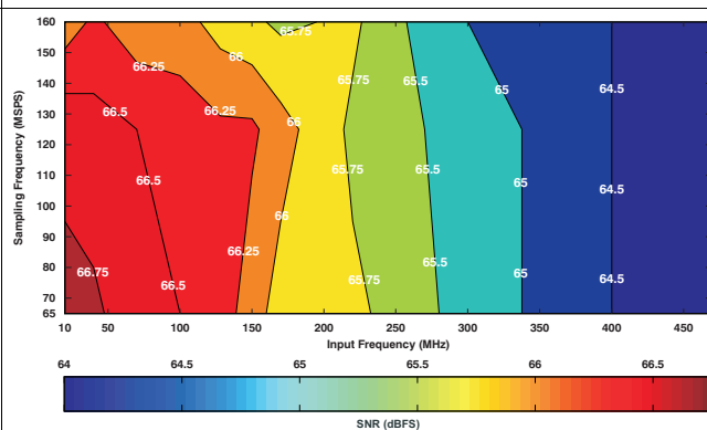
Figure 134. ADS422x Signal-to-Noise Ratio (6-dB Gain)
