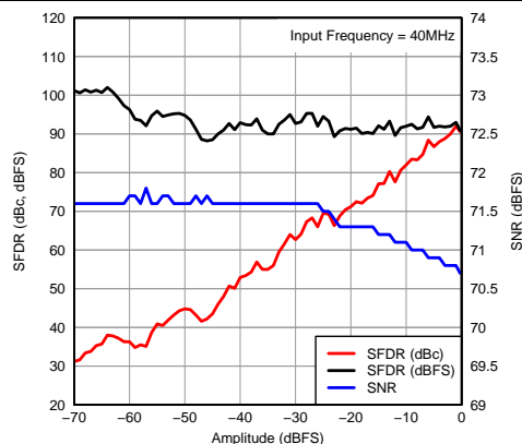
Figure 95. Performance vs Input Amplitude
