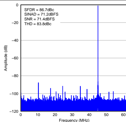
Figure 29. FFT for 170-MHz Input Signal
