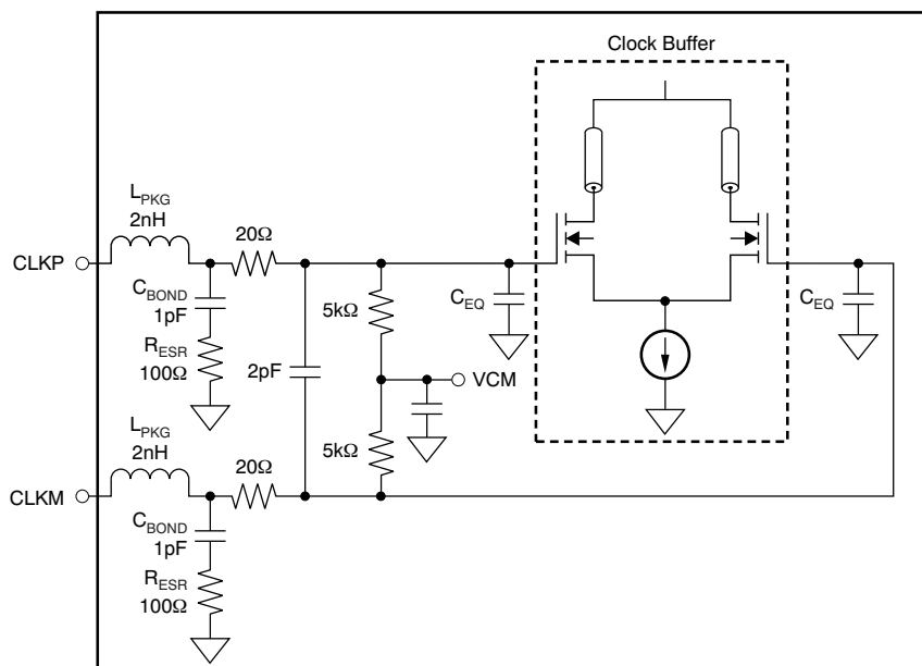
Figure 147. Internal Clock Buffer
