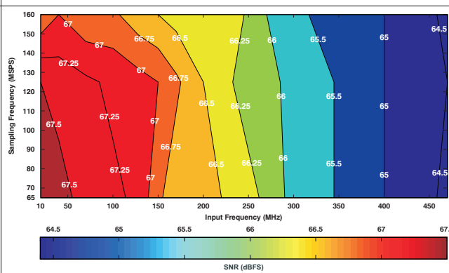
Figure 132. ADS424x Signal-to-Noise Ratio (6-dB Gain)
