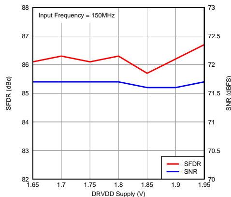
Figure 43. Performance vs DRVDD Supply Voltage
