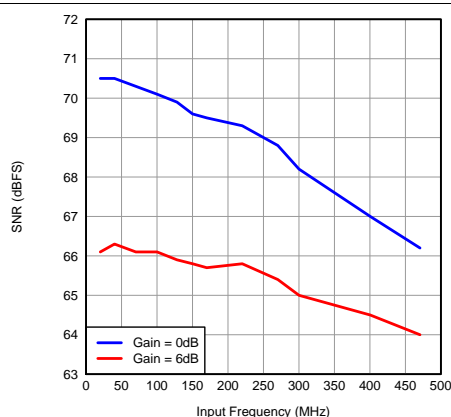
Figure 92. SNR vs Input Frequency
