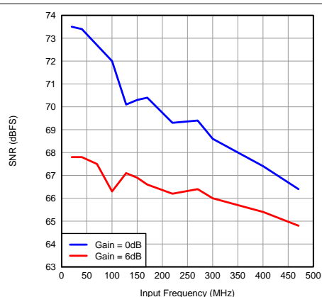
Figure 55. SNR vs Input Frequency (CMOS)
