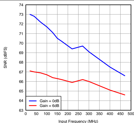
Figure 13. SNR vs Input Frequency (CMOS)
