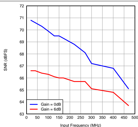
Figure 93. SNR vs Input Frequency (CMOS)
