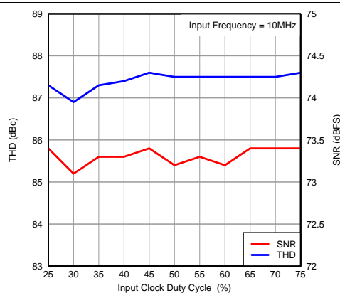
Figure 45. Performance vs Input Clock Duty Cycle
