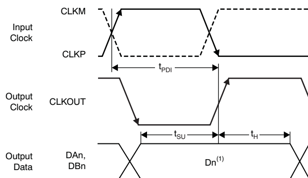
Figure 1. CMOS Interface Timing Diagram
