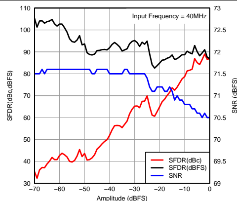
Figure 79. Performance vs Input Amplitude
