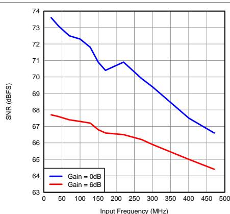
Figure 54. SNR vs Input Frequency
