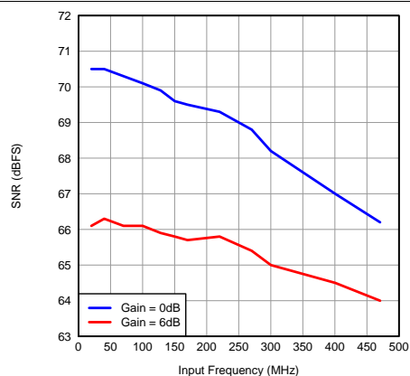
Figure 75. SNR vs Input Frequency
