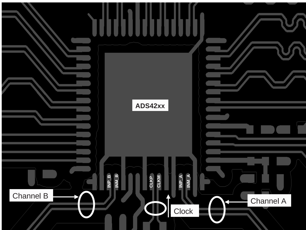
Figure 164. ADS42xx EVM PCB Layout
