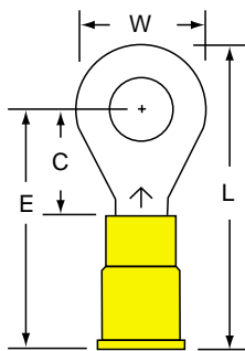
MV10-14R/S Stud Size 1/4 Wire Range 12-10
