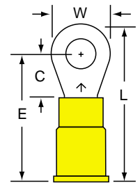
MV10-10R Stud Size 10 Wire Range 12-10
