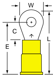
MV10-6R Stud Size 6 Wire Range 12-10
