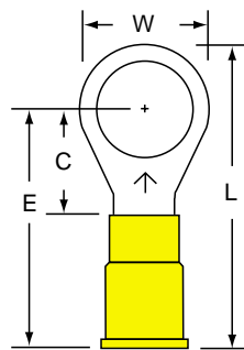
MV10-38R/S Stud Size 3/8 Wire Range 12-10
