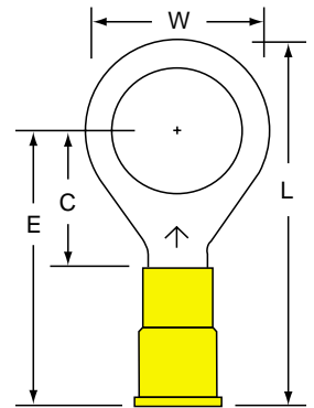
MV10-12R Stud Size 1/2 Wire Range 12-10
