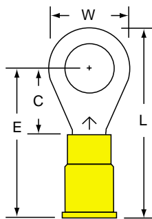
MV10-516R/S Stud Size 5/16 Wire Range 12-10
