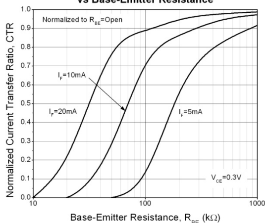
Figure 4. Current Transfer Ratio (Saturated) vs Base-Emitter Resistance
