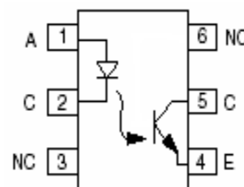
CNY17F-X
