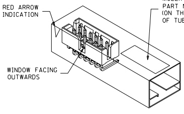
FIG.1 : ORIENTATION OF PART IN TUBE. (FOR THE REFERENCE OF PART/TUBE ASSEMBLY.)
