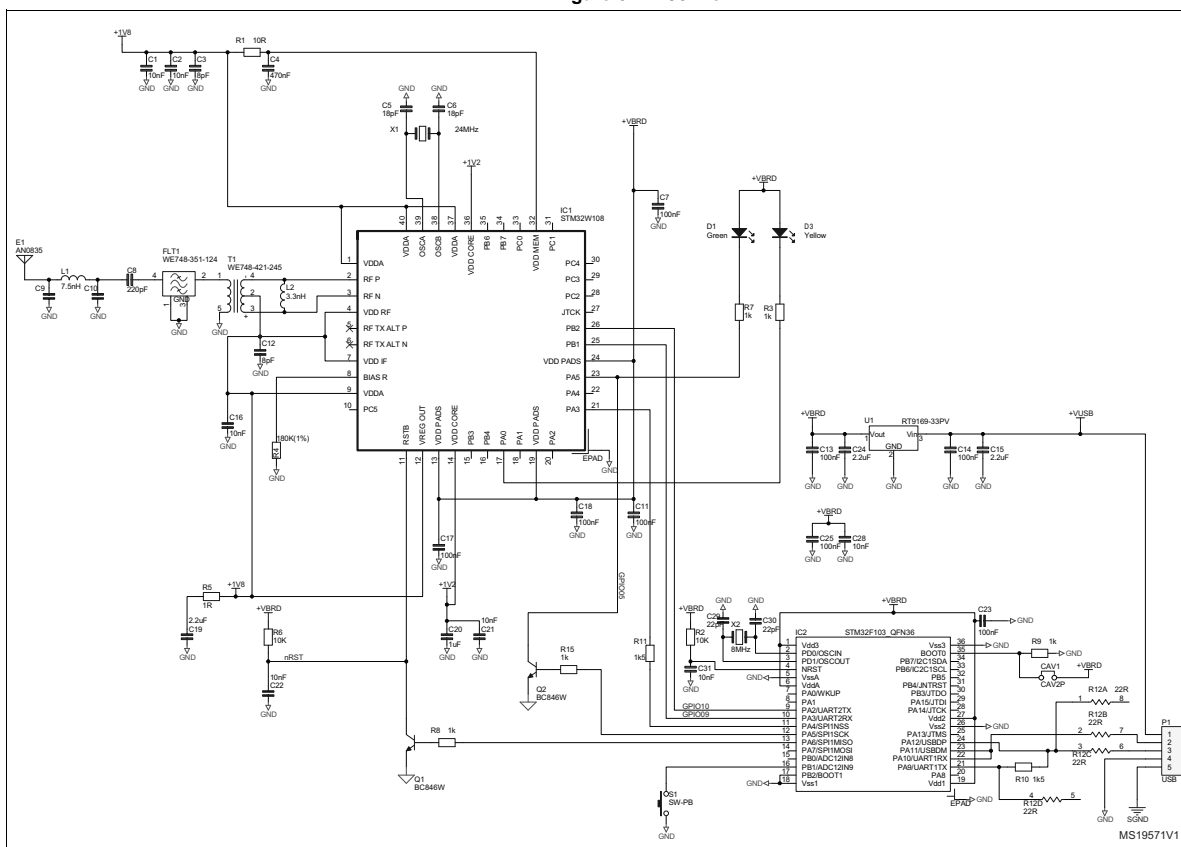
Figure 6. MB951 rev. A
