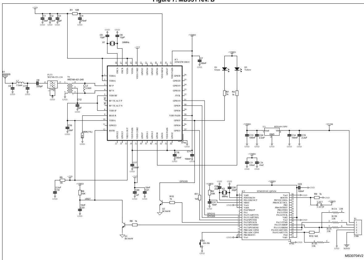
Figure 7. MB951 rev. B
