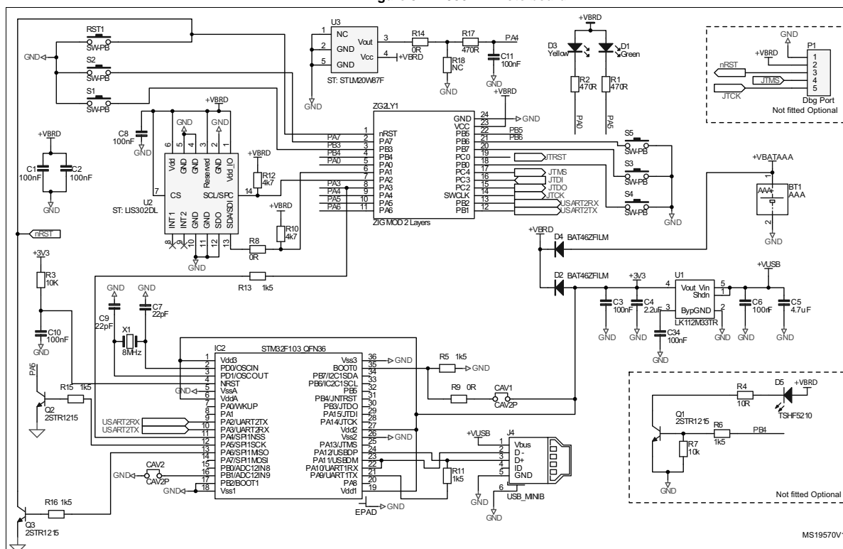
Figure 5. MB950 RF-mote board
