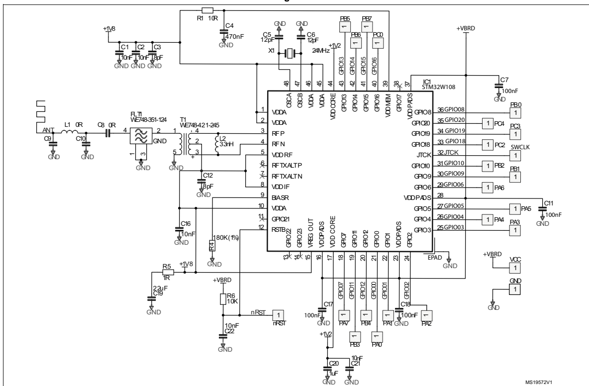
Figure 3. MB953 rev. A
