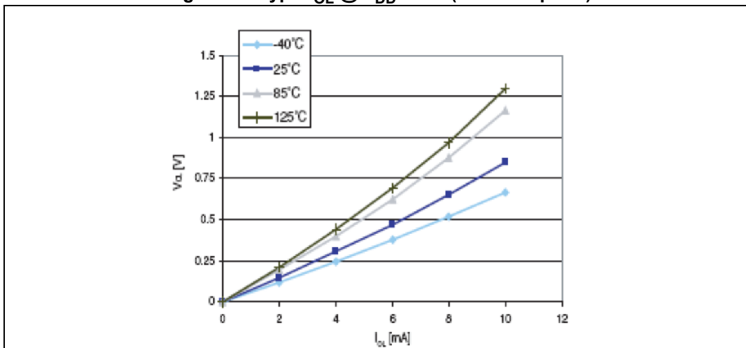
Figure 22. Typ. V_{OL} @ V_{DD} = 5 \text{ V} (standard ports)
