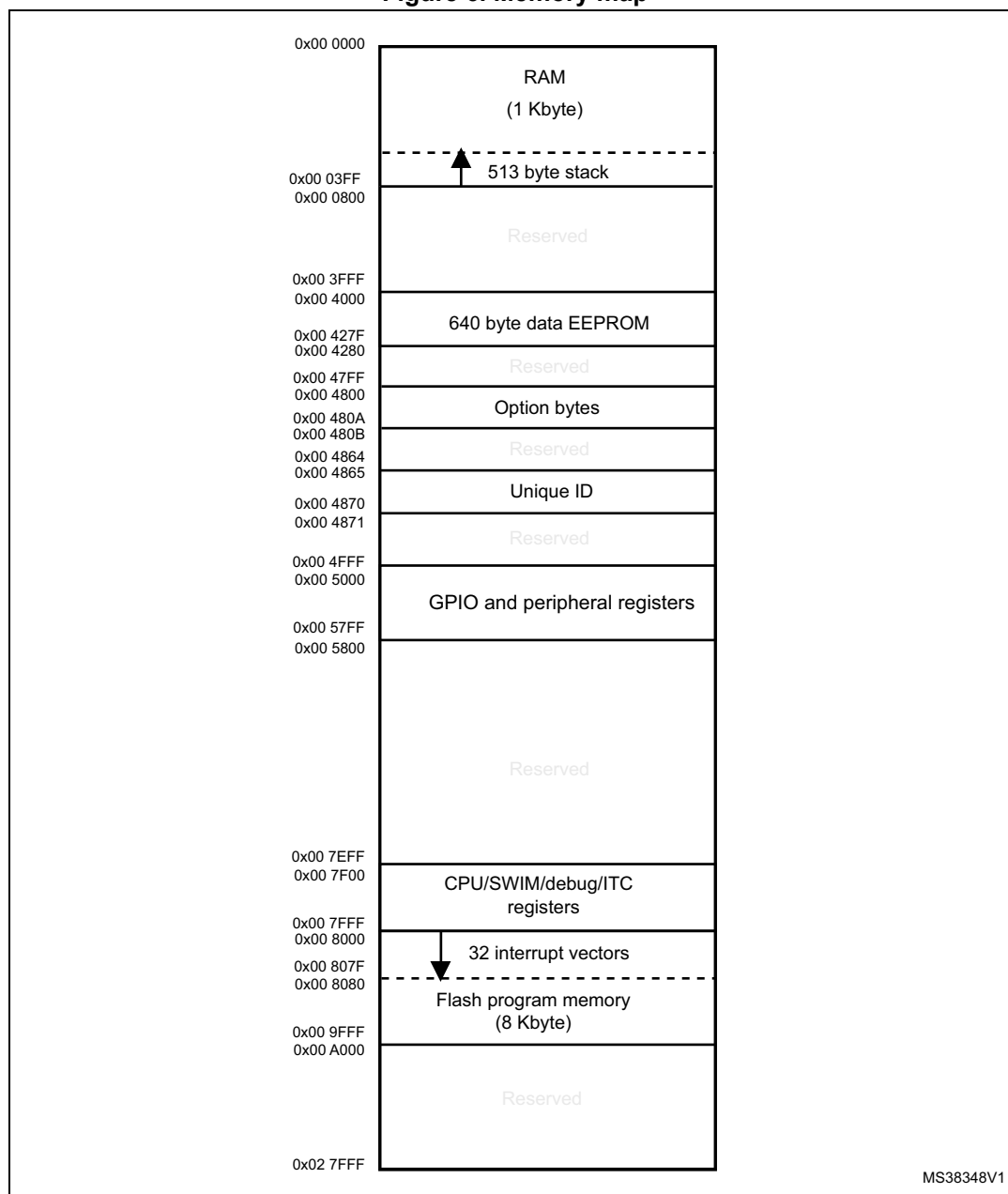
Figure 6. Memory map
