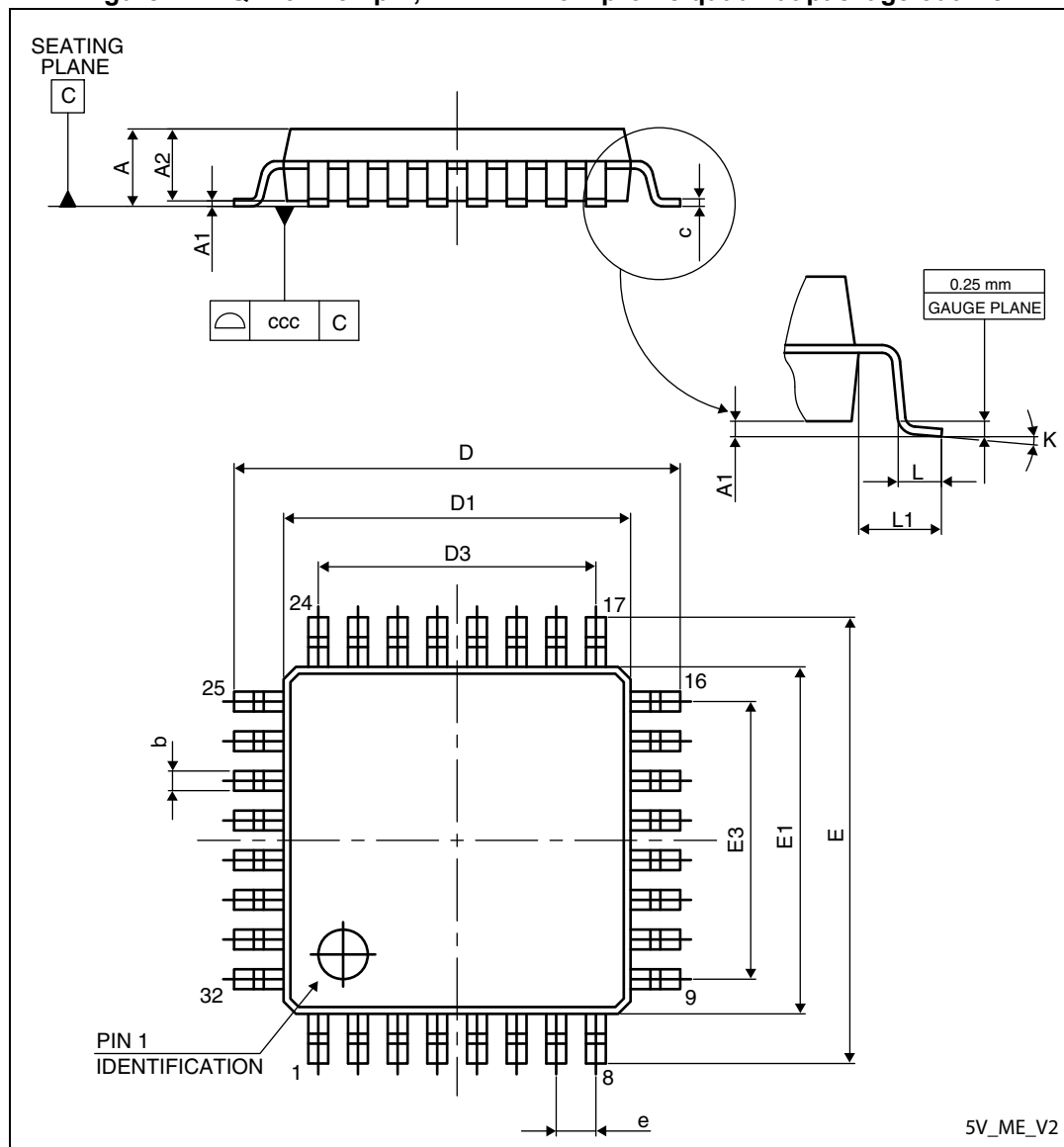
Figure 42. LQFP32 - 32-pin, 7 x 7 mm low-profile quad flat package outline
