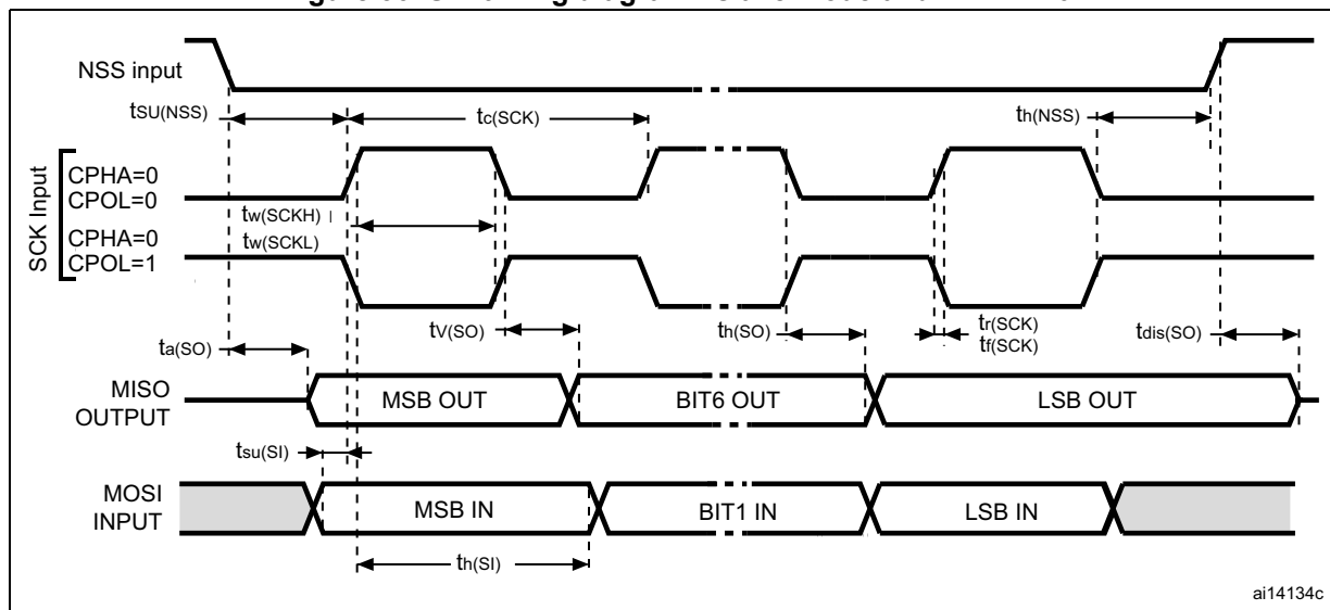
Figure 36. SPI timing diagram - slave mode and CPHA = 0
