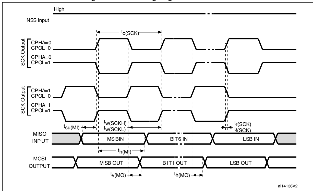
Figure 36. SPI1 timing diagram - master mode
