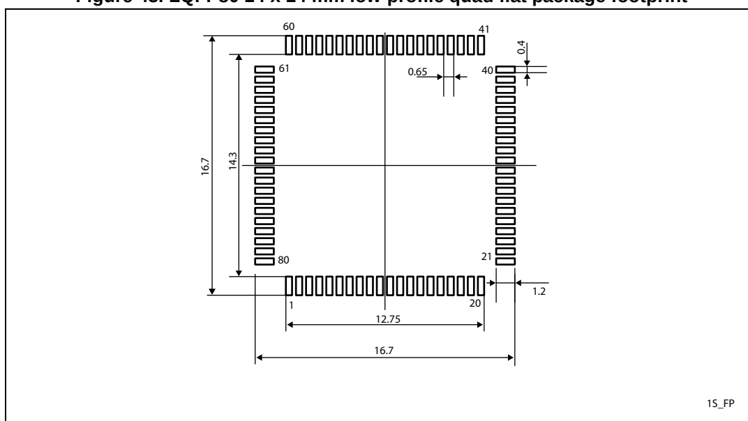
Figure 43. LQFP80 14 x 14 mm low-profile quad flat package footprint
