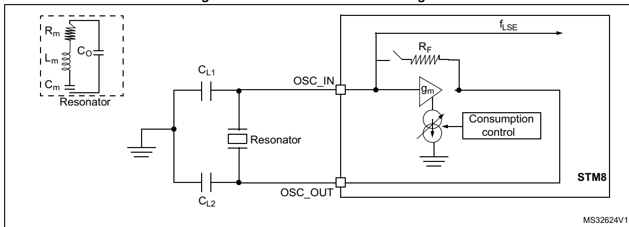
Figure 18. LSE oscillator circuit diagram
