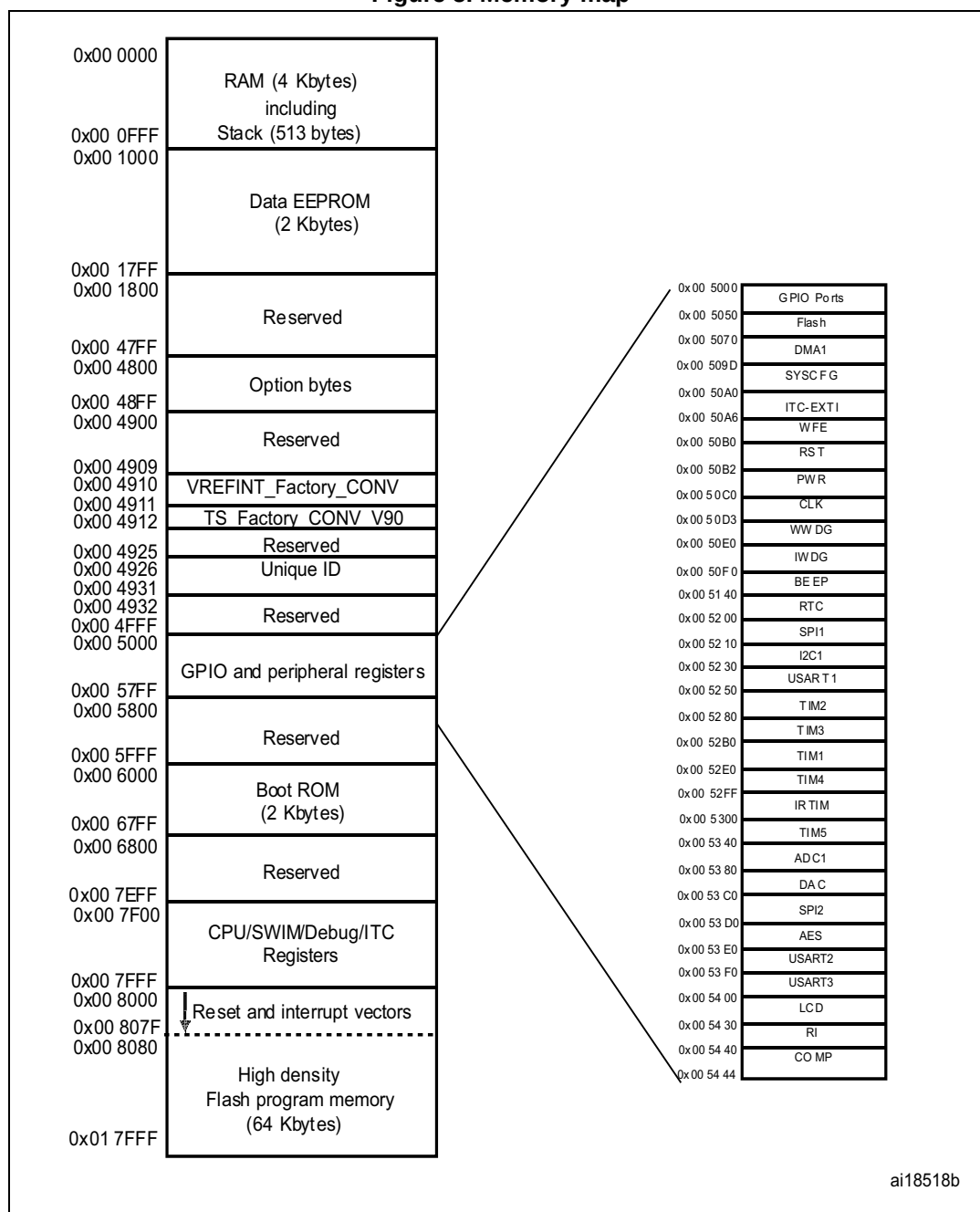
Figure 5. Memory map
