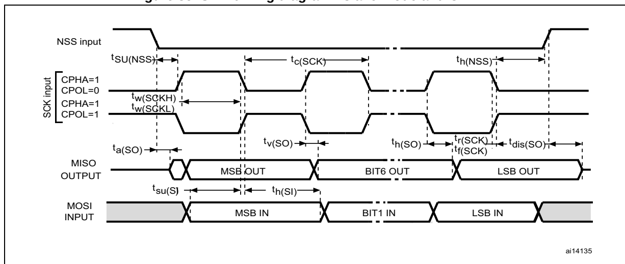
Figure 35. SPI1 timing diagram - slave mode and CPHA=1
