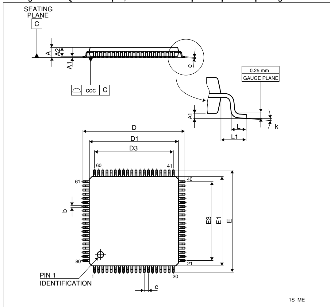
Figure 42. LQFP80 - 80-pin, 14 x 14 mm low-profile quad flat package outline
