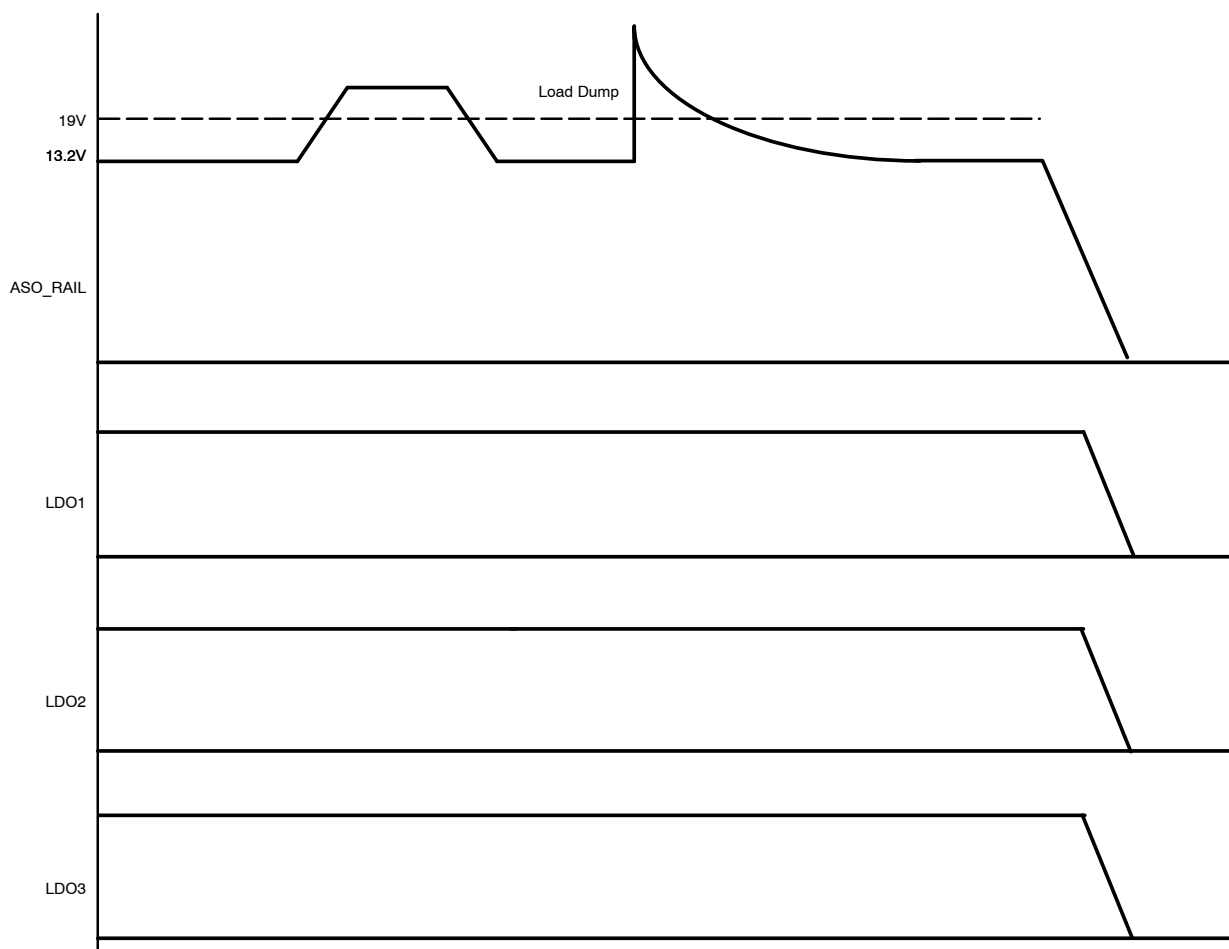
Figure 11. NCV8612B Regulator Output Timing Diagram– VBATT_MON Grounded
