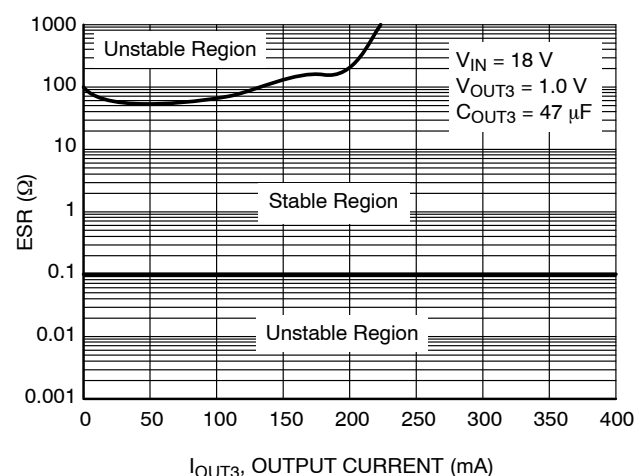
Figure 27. C OUT3 ESR Stability Region – 47 \mu F
