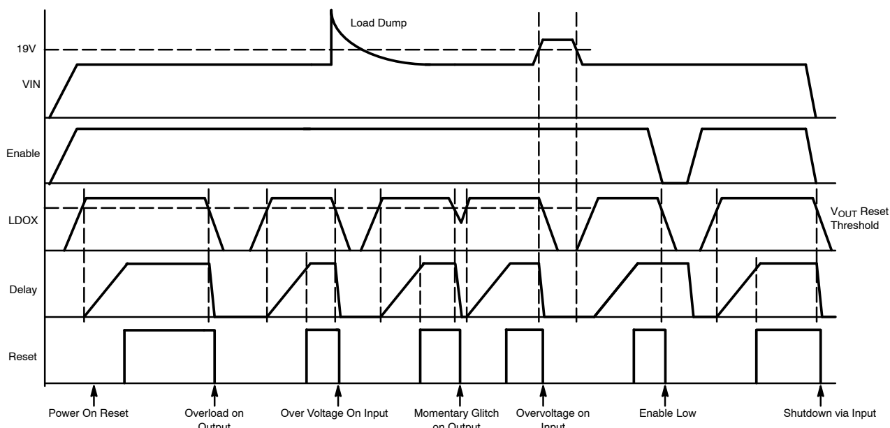
Figure 5. NCV8612B Reset Timing Diagram
