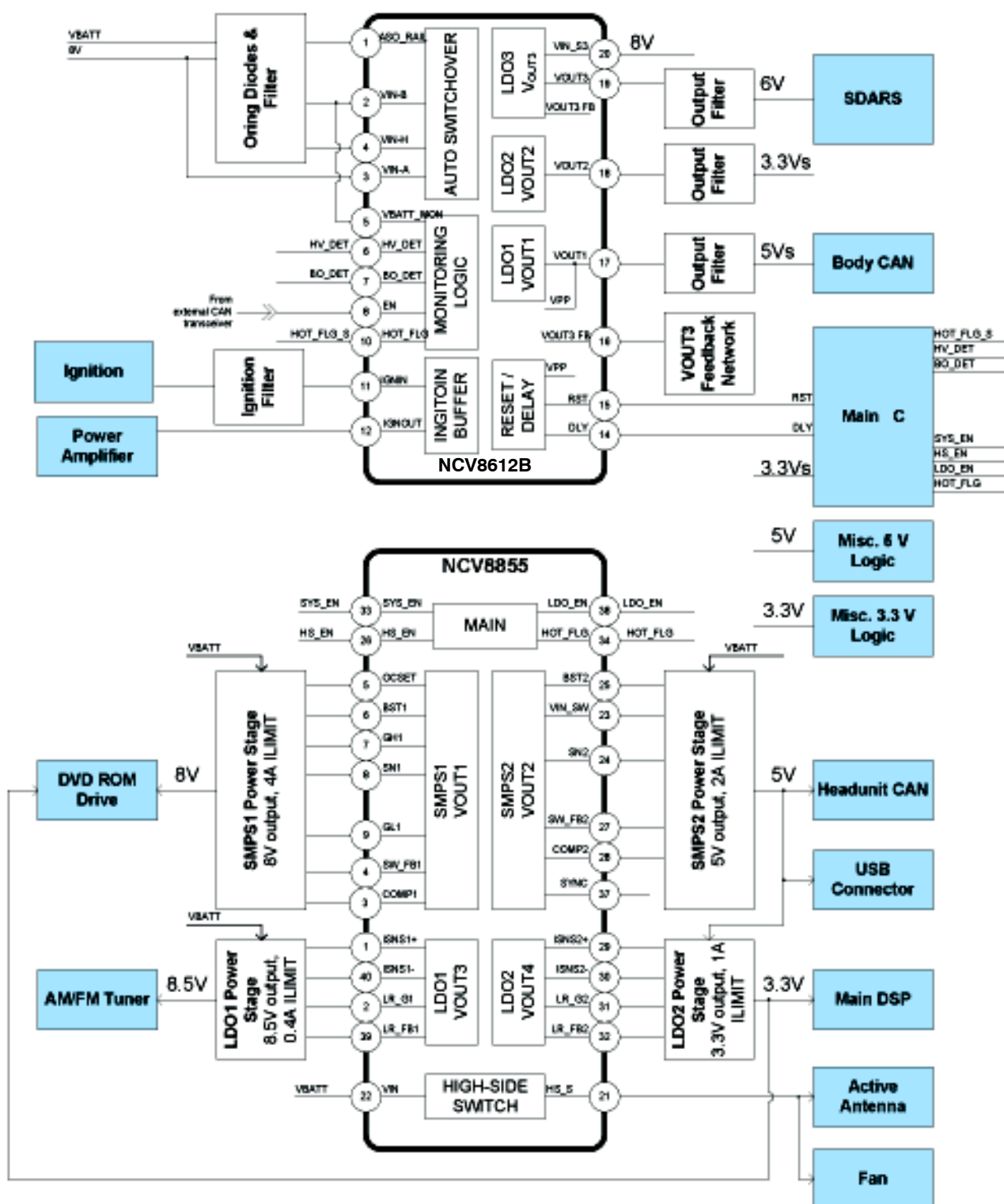
Figure 2. Automotive Radio System Block Diagram Example NCV8612B with NCV8855
