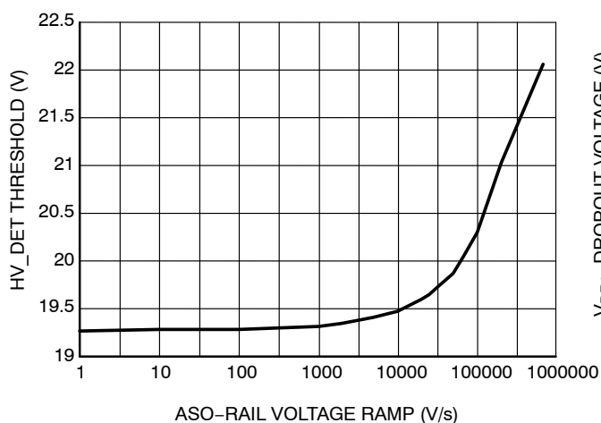
Figure 18. HV-DET Threshold vs. dV/dt
