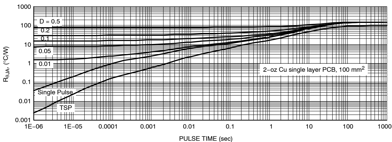
Figure 21. R_{\theta JA} vs. Duty Cycle
