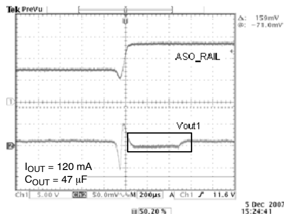
Figure 3. V OUTX Response to ASO Switchover Event
