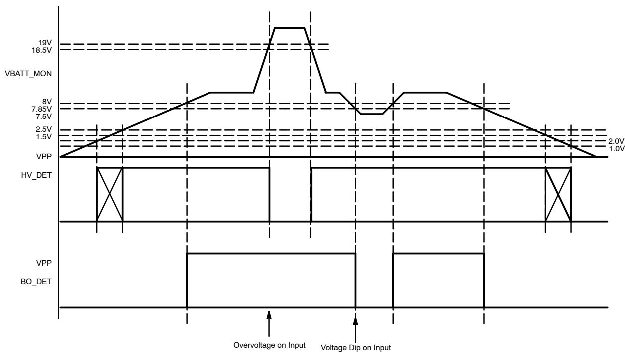
Figure 8. Warning Circuitry Timing Diagram
