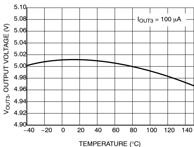
Figure 14. Output Voltage LDO3 vs Temperature
