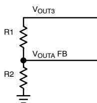
Figure 4. Feedback Network
