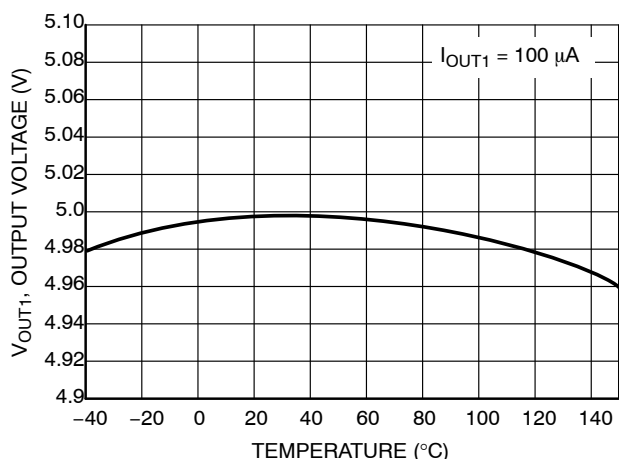
Figure 12. Output Voltage LDO1 vs Temperature
