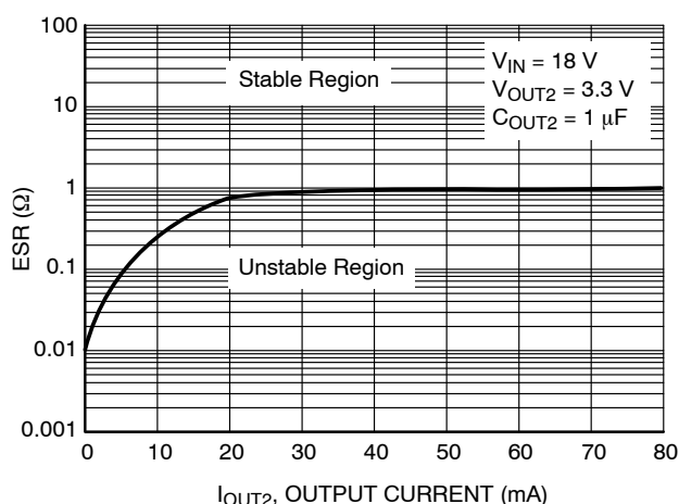
Figure 24. C OUT2 ESR Stability Region – 1 \mu F
