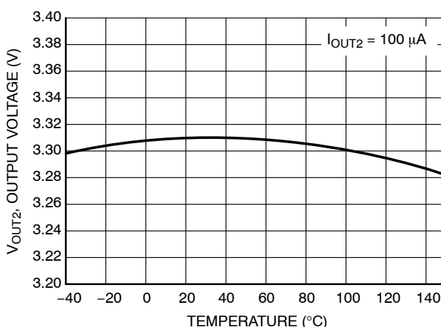
Figure 13. Output Voltage LDO2 vs Temperature
