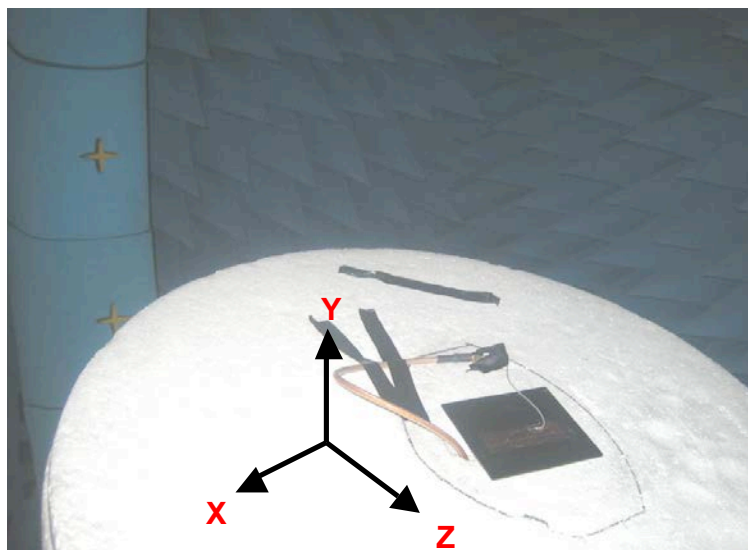
Figure 1. Satimo System.
