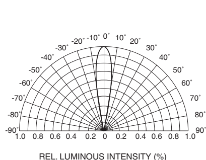
Fig.4 Radiation Diagram
