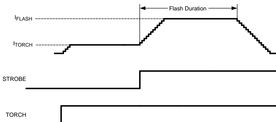
Figure 26. Hardware-Torch Mode
