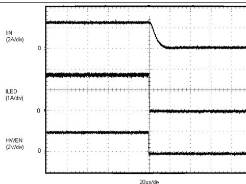
Figure 20. NTC-Mode Operation
