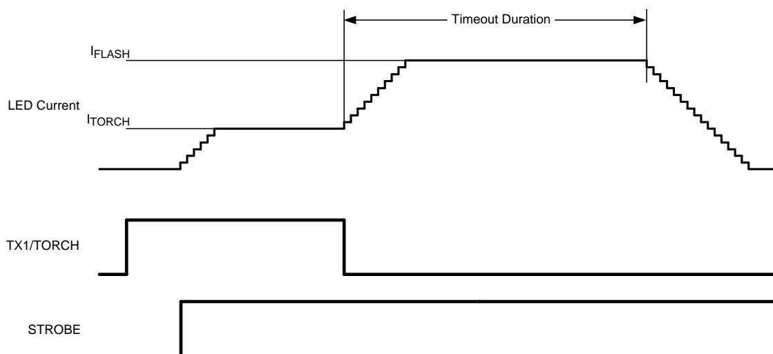
Figure 38. AET Mode Timing
