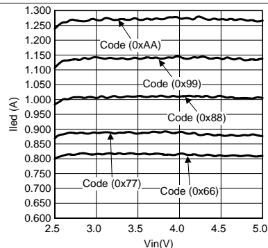
Middle 5 Flash Brightness Codes
