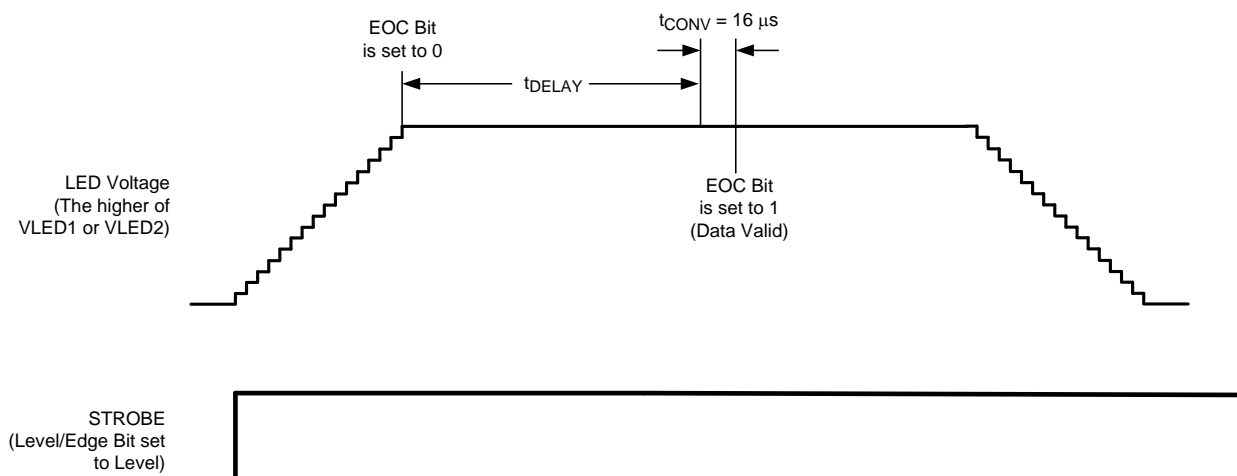
Figure 32. V_{\text{LED}} Monitor Automatic Mode
