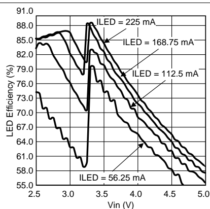
Figure 45. LED Efficiency vs V_{IN} Dual LEDs
