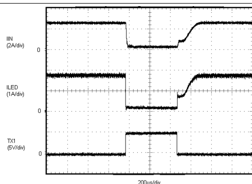
Figure 21. AET-Mode Operation
