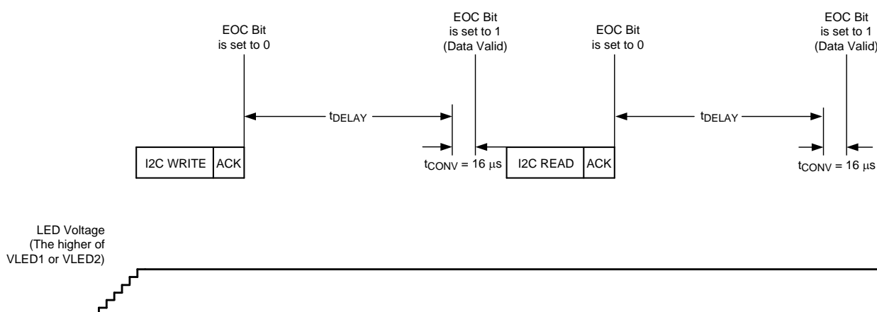
Figure 33. V_{\text{LED}} Monitor Manual Mode
