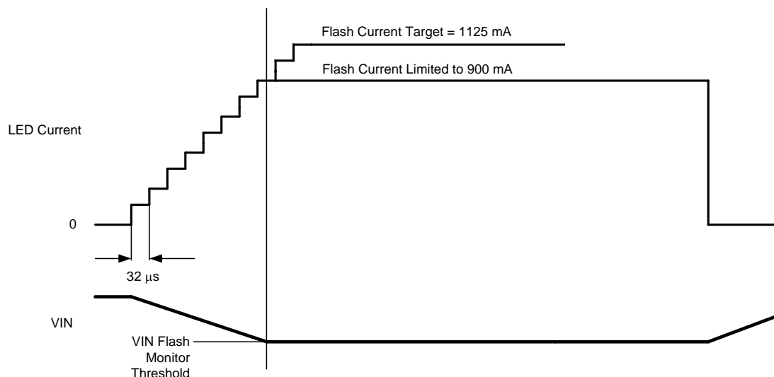
Figure 31. V_{IN} Flash Monitor Example
