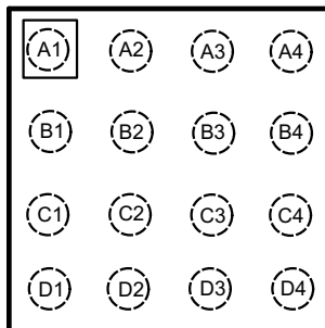
Pin Functions
