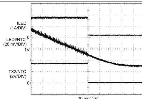
Figure 20. NTC-Mode Operation
