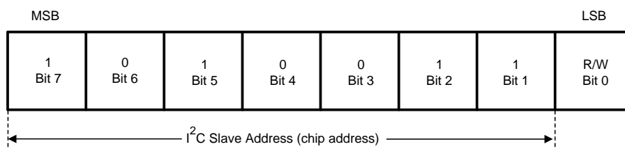
Figure 41. Device Address
