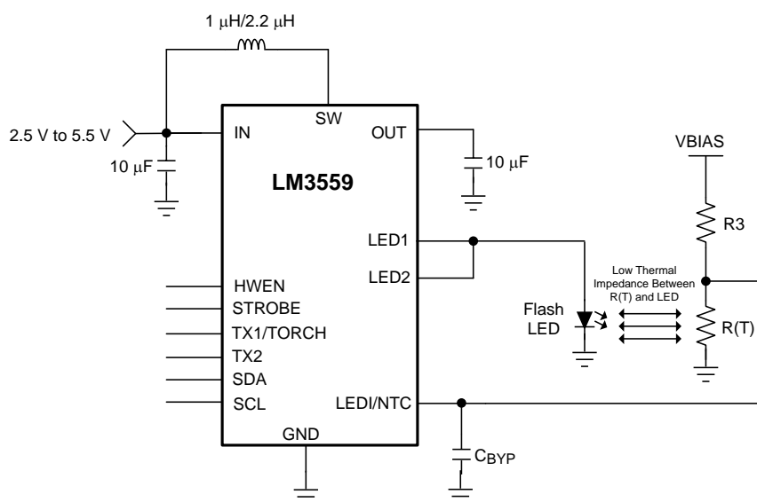
Figure 48. LM3559 Typical Application Circuit With Thermistor
