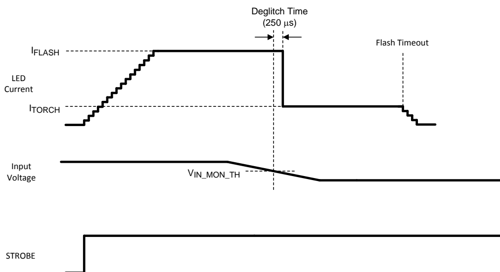
Figure 30. V_{IN} Monitor Waveform
