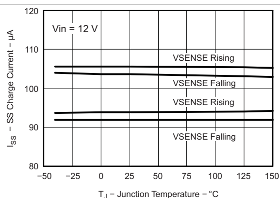
Figure 12. PWRGD Threshold vs Temperature
