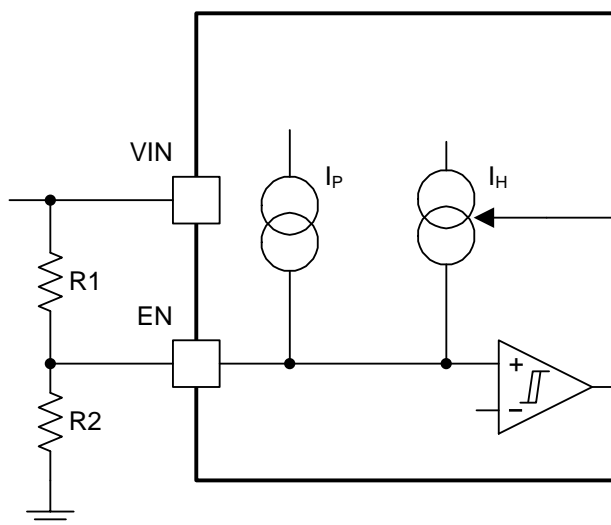
Figure 17. Adjustable VIN Undervoltage Lockout
