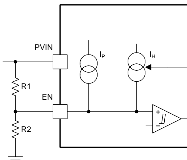
Figure 18. Adjustable PVIN Undervoltage Lockout, VIN ≥ 4.5 V
