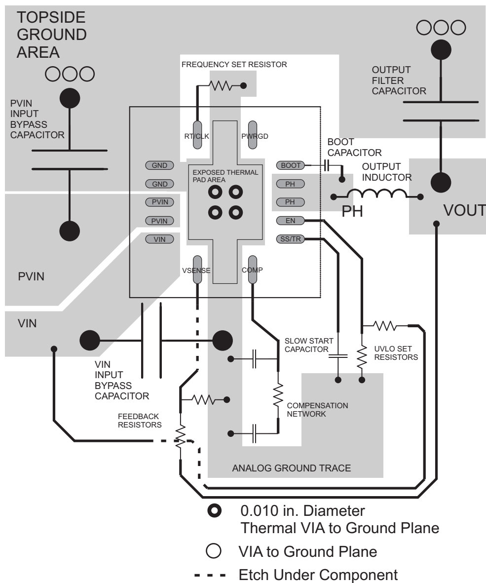
Figure 46. PCB Layout
