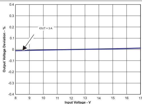
Figure 37. Line Regulation
