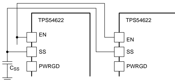
Figure 27. Ratiometric Start-Up Sequence
