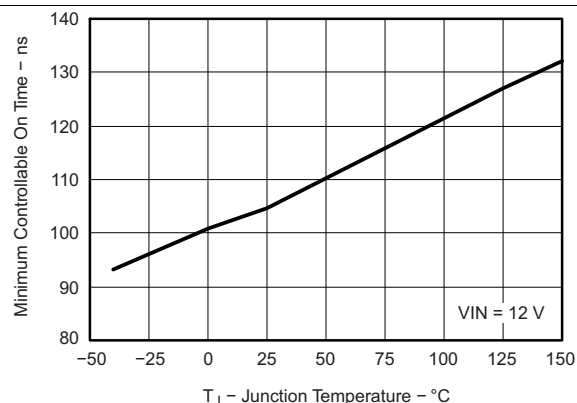
Figure 14. Minimum Controllable On-Time vs Temperature
