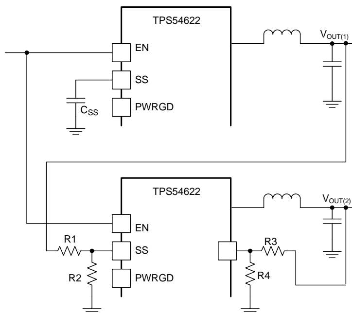
Figure 28. Ratiometric and Simultaneous Start-Up Sequence
