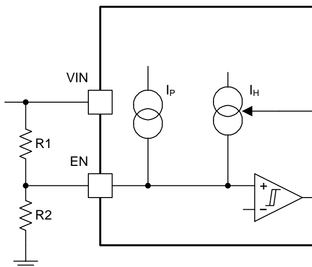
Figure 19. Adjustable VIN and PVIN Undervoltage Lockout
