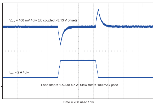
Figure 30. Load Transient
