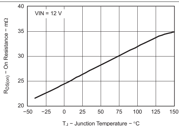
Figure 1. High-Side R_{DS(on)} vs Temperature
