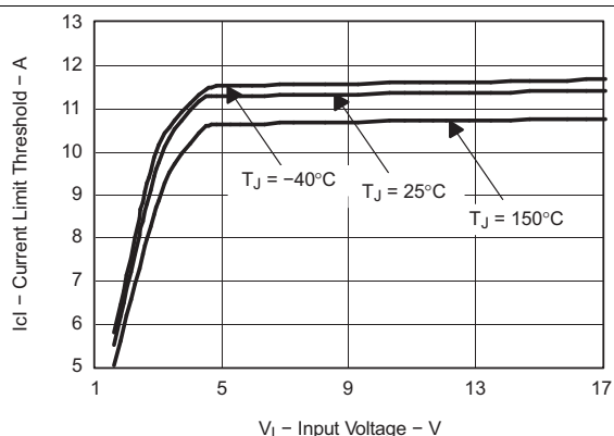
Figure 13. High-Side Current Limit Threshold vs Input Voltage
