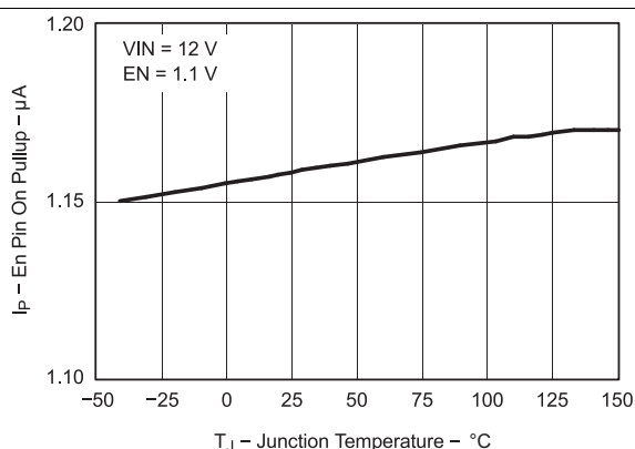
Figure 7. Pin Pull-Up Current vs Temperature
