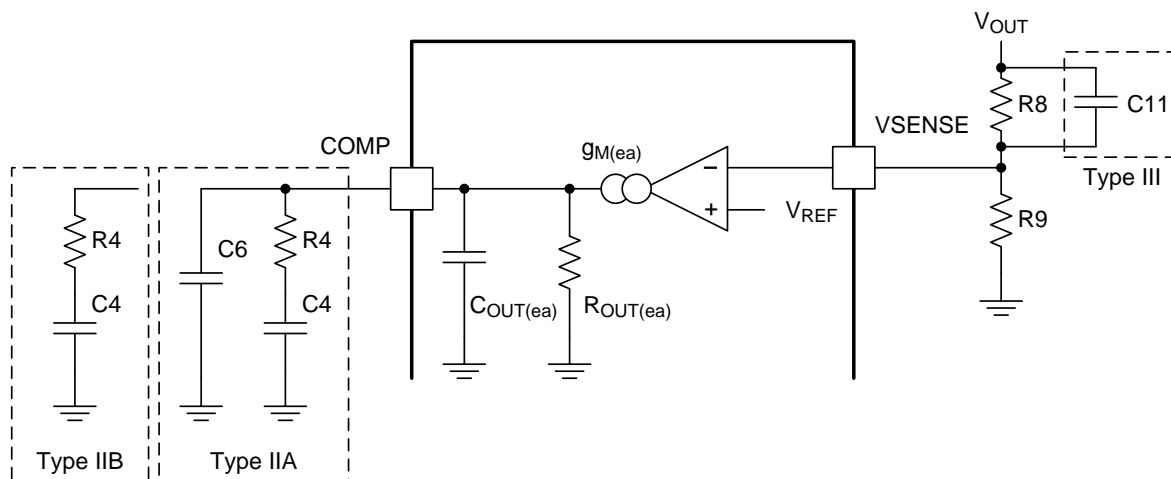
Figure 23. Types of Frequency Compensation
