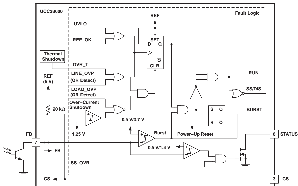
Figure 8. Fault Logic Details
