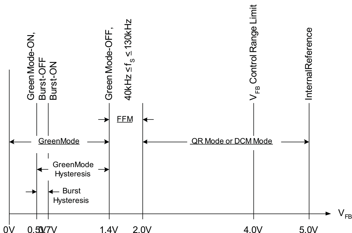
Figure 2. Mode Control with FB Pin Voltage
