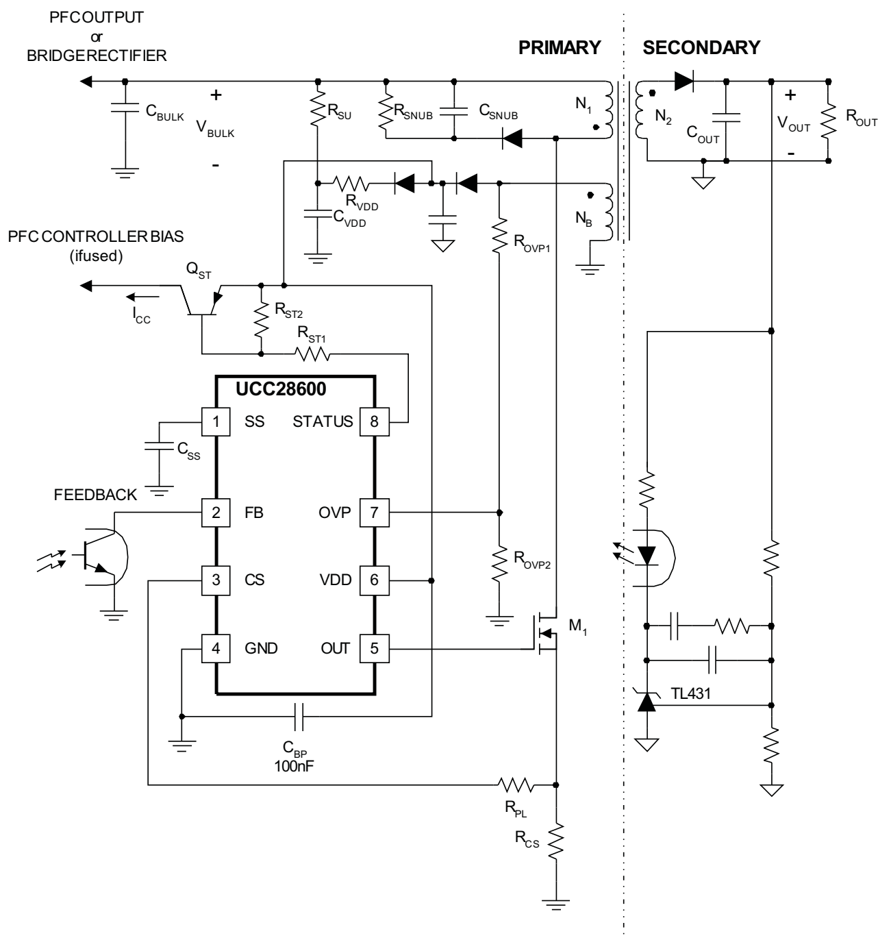
Figure 1. Pin Termination Schematic
