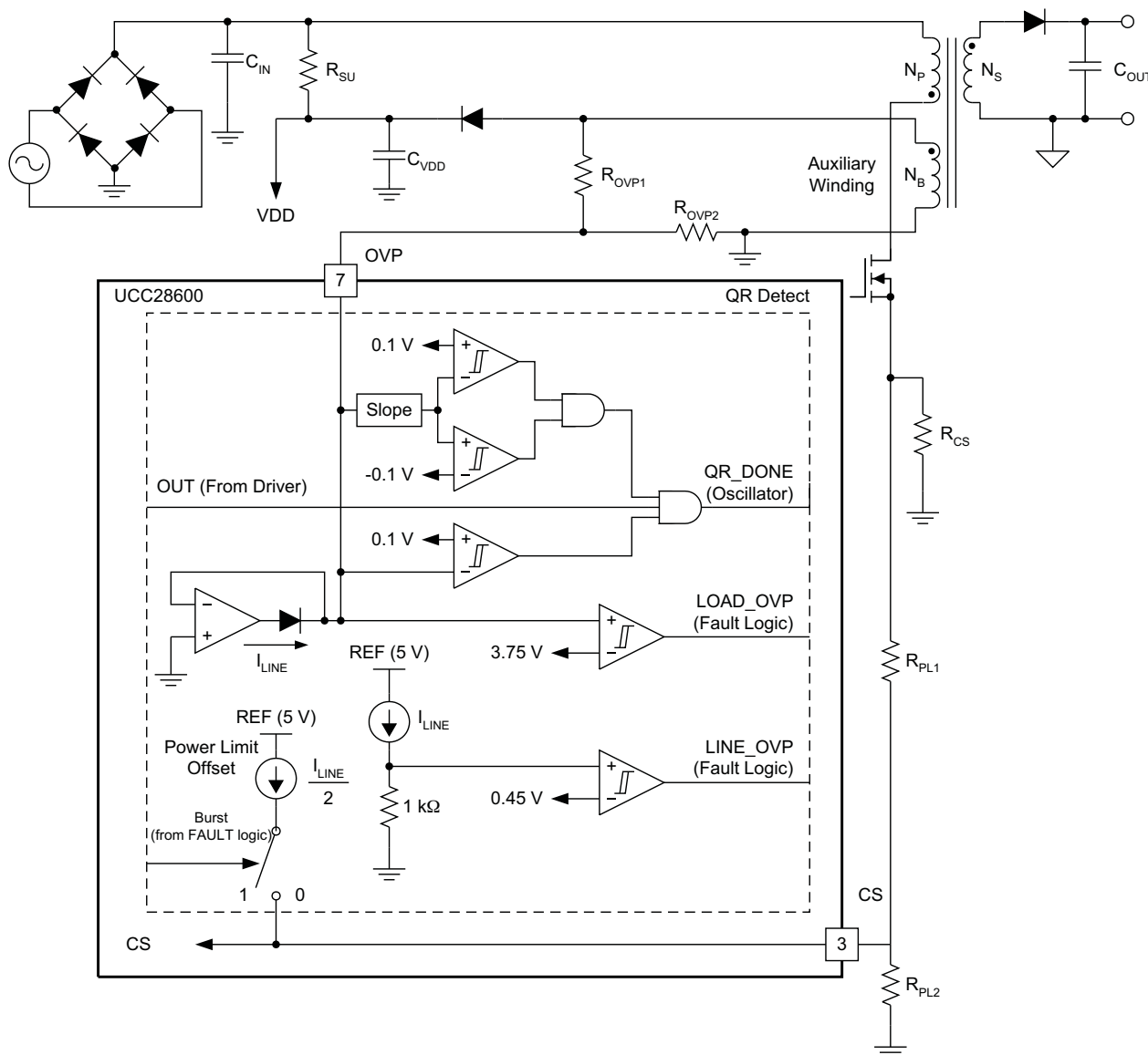
Figure 7. QR Detect Details
