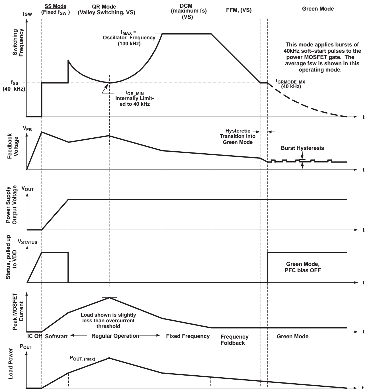
Figure 4. Operation Mode Switching Frequencies
