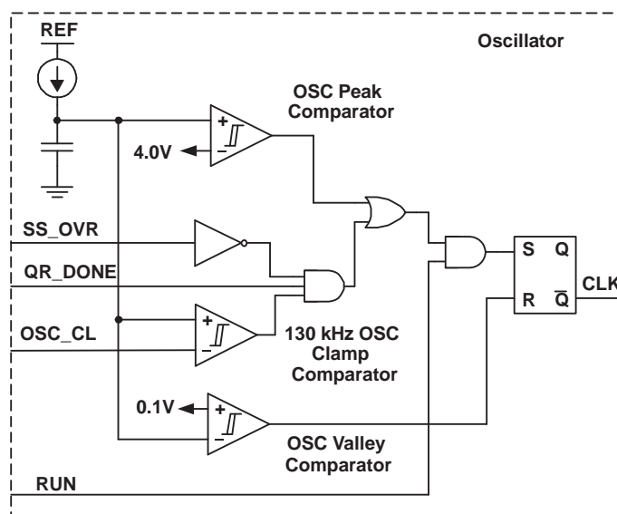
Figure 5. Oscillator Details
