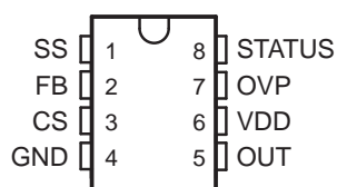
UCC28600 D PACKAGE (TOP VIEW)
