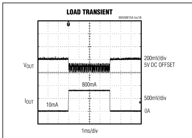
Figure 2. Load Regulation
