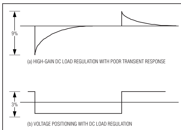
Figure 3. Transient-Response Comparison
