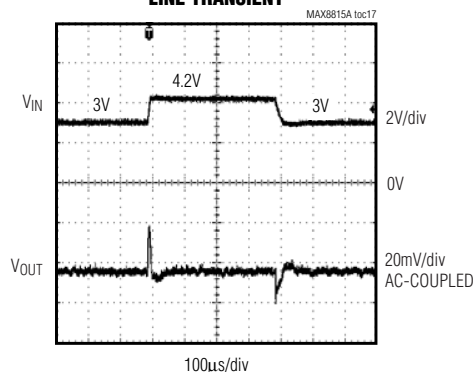
LINE TRANSIENT
