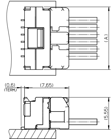
嵌合図 MATED CONNECTORS
