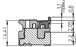
SECTION Z-Z
