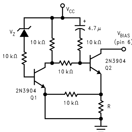
Figure 45. External Undervoltage Pull-Down
