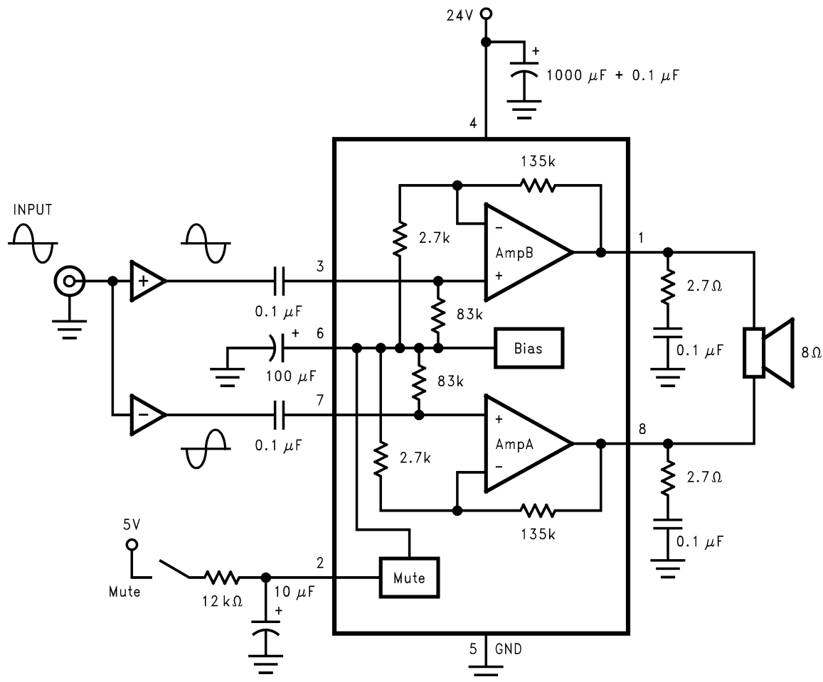
Figure 43. Bridge-Mode Application
