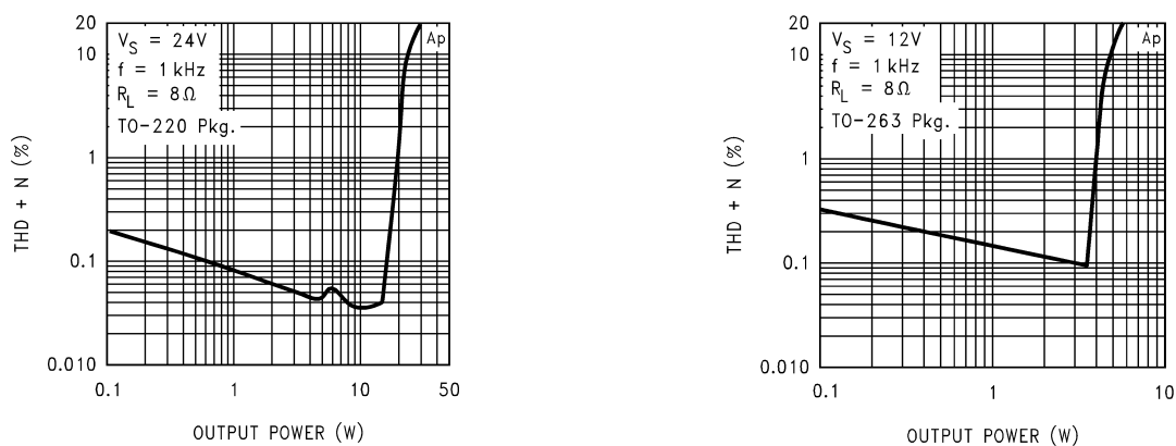
Figure 44. THD+N vs P_{OUT} for Bridge-Mode Application
