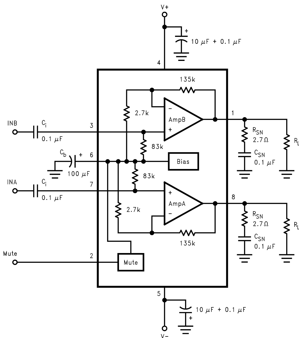
Figure 3. Test Circuit
