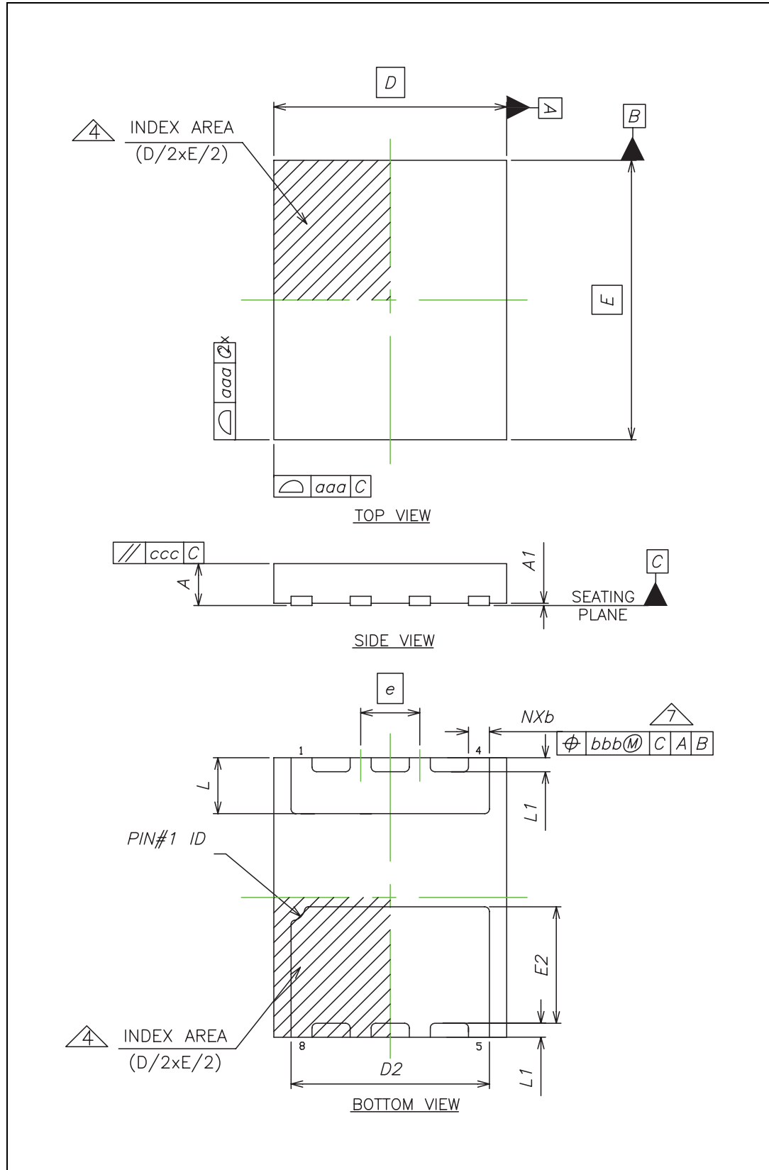
Figure 5. PQFN 5 x 6 mm drawing
