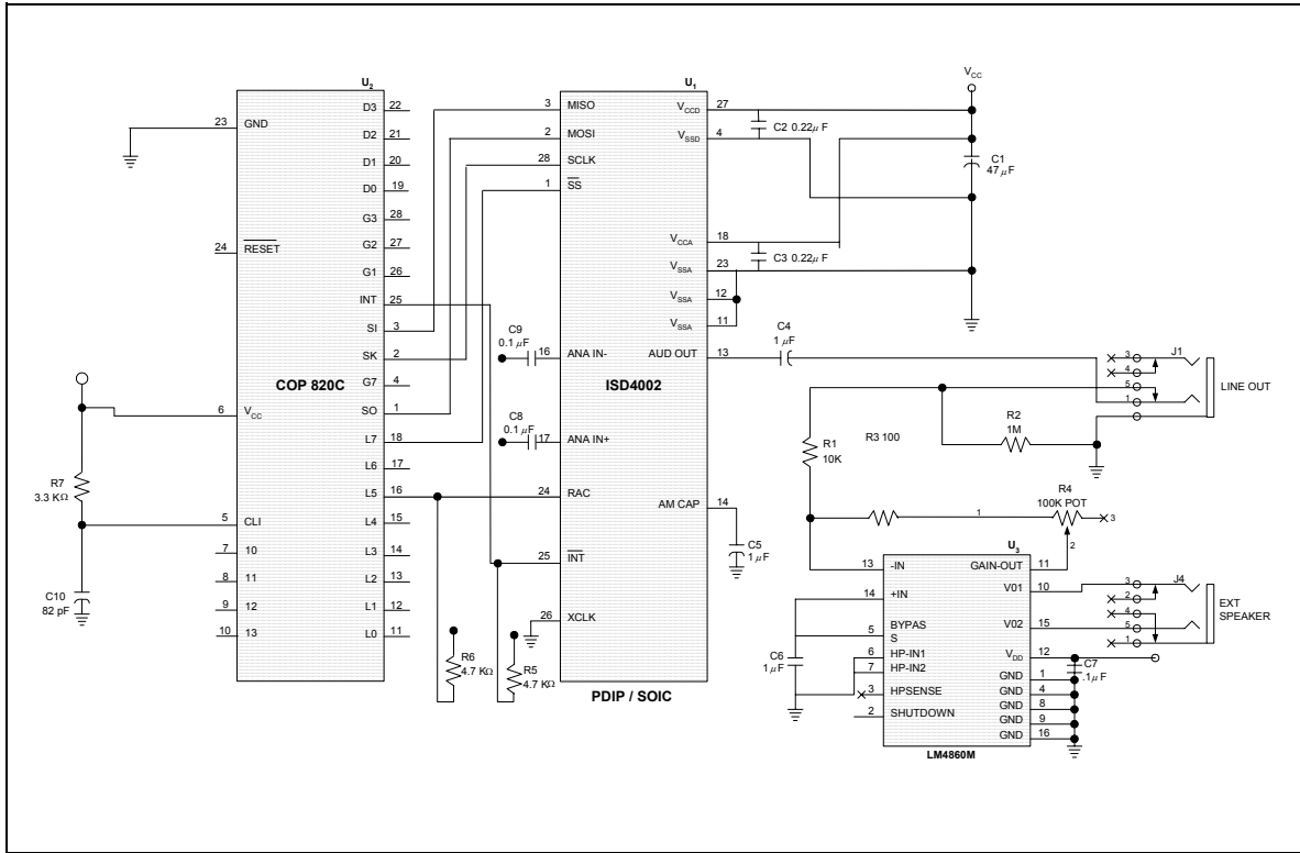
FIGURE 11: APPLICATION EXAMPLE USING SPI PORT ON MICROCONTROLLER
