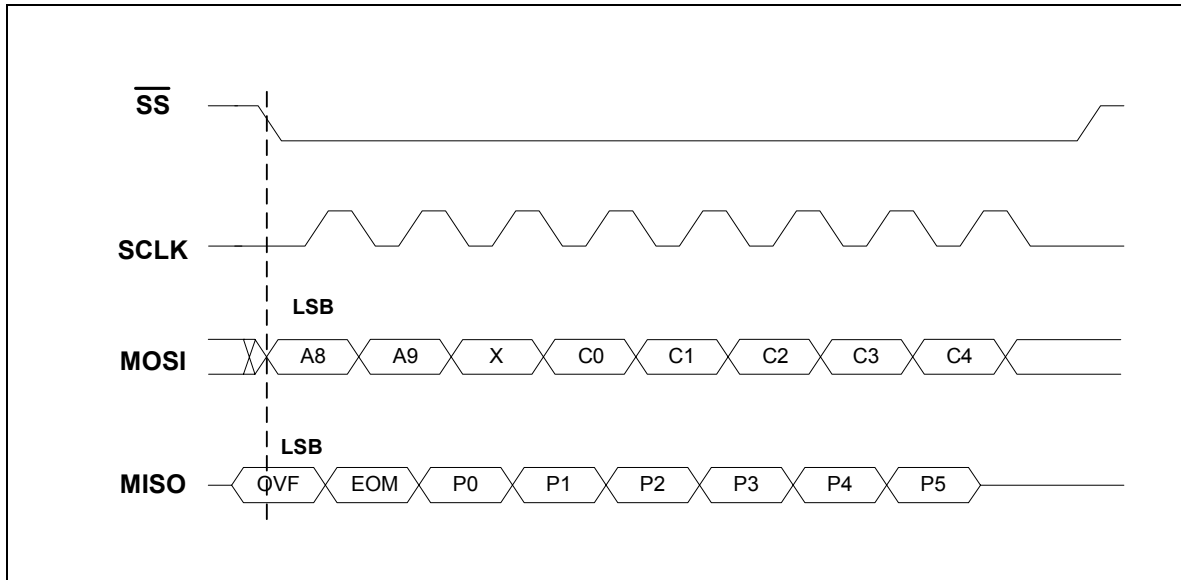
FIGURE 6: 8-BIT COMMAND FORMAT
