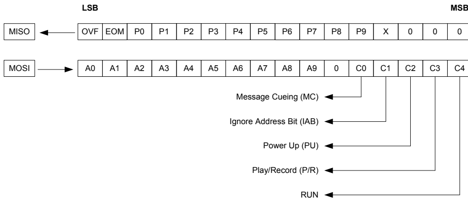
FIGURE 4: SPI PORT
