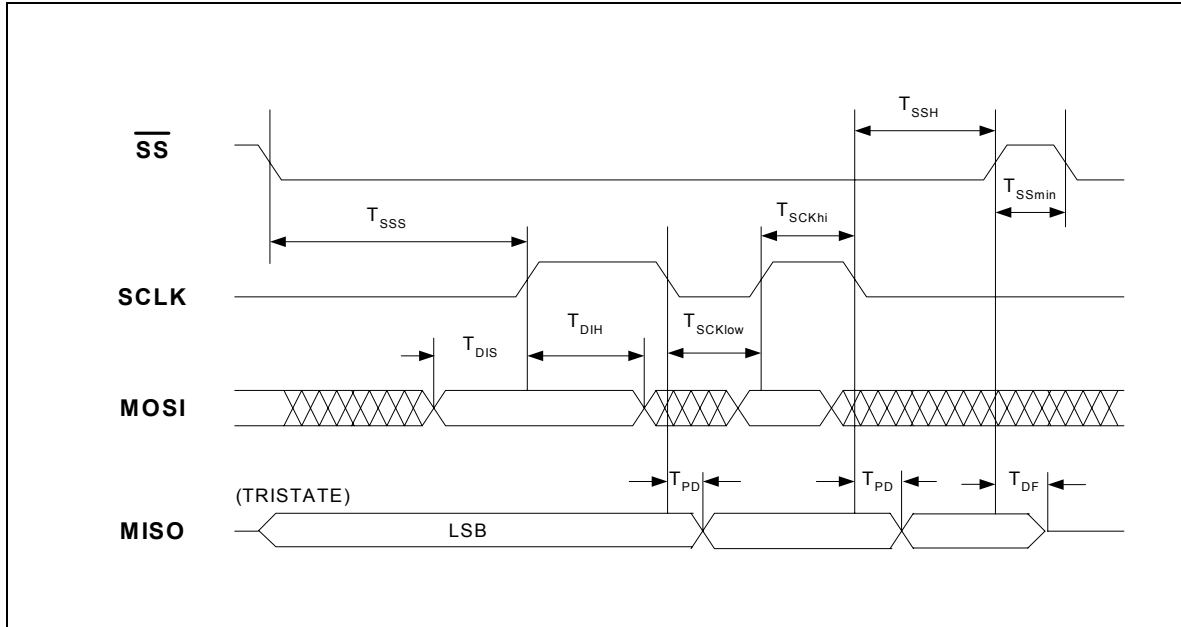
FIGURE 5: TIMING DIAGRAM
