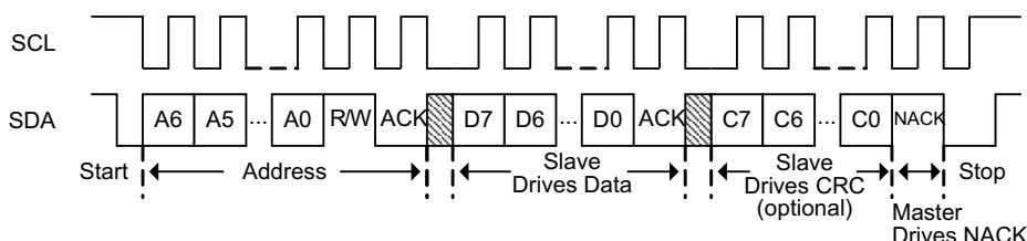
Figure 14. I 2 C Read Command
