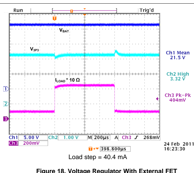
Figure 18. Voltage Regulator With External FET
