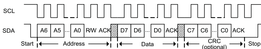
Figure 13. I 2 C Write Command
