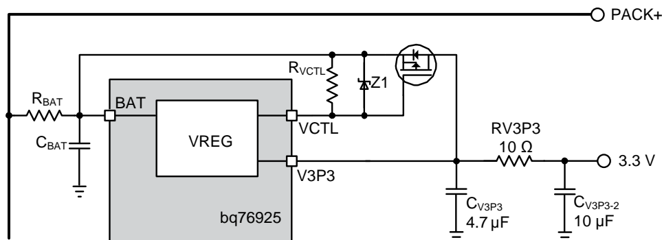
Figure 15. LDO Regulator
