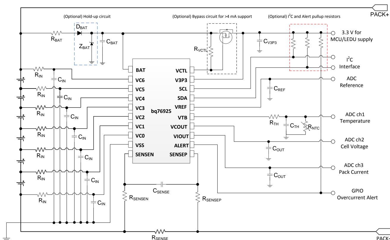
Figure 16. Typical Schematic
