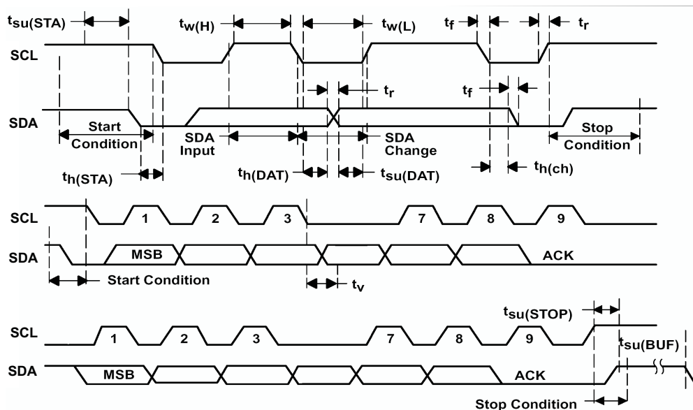
Figure 1. I 2 C Timing
