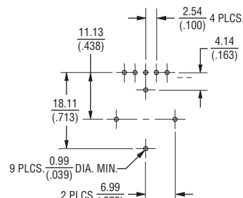
Recommended Board Layout with Bracket
