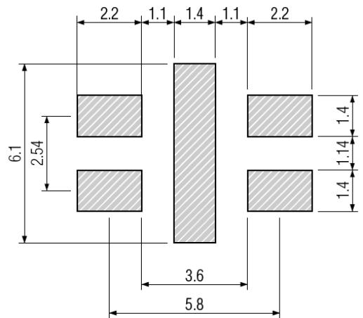
Figure 2) Land Pattern
