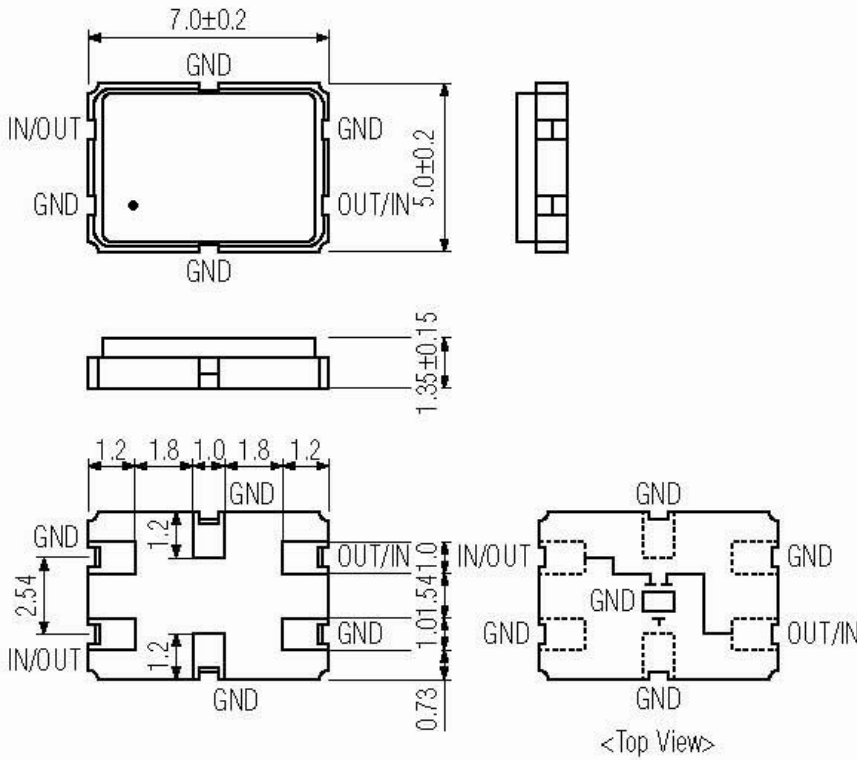
Figure 1) Top, Side and Bottom Views
