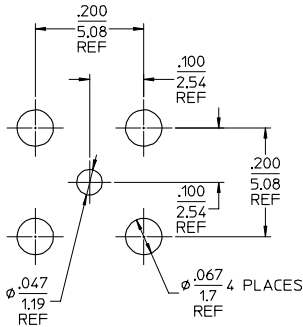
RECOMMENDED BOARD LAYOUT
