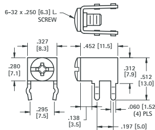
7692-2 SNAP-IN PC MOUNT
