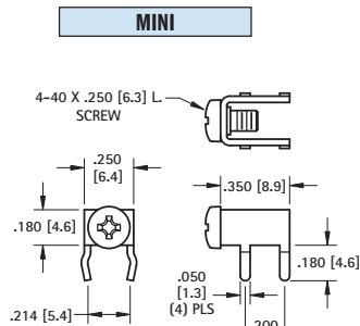
7773 SNAP-IN PC MOUNT
