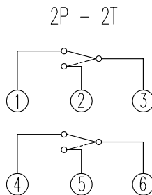
(VIEWED FROM DIRECTION C)
