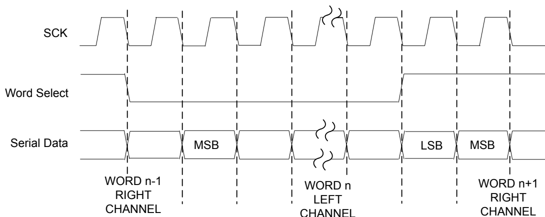
Figure 16-3. Left-Justified Data Transfer
