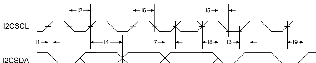
Figure 25-17. I 2 C Timing
