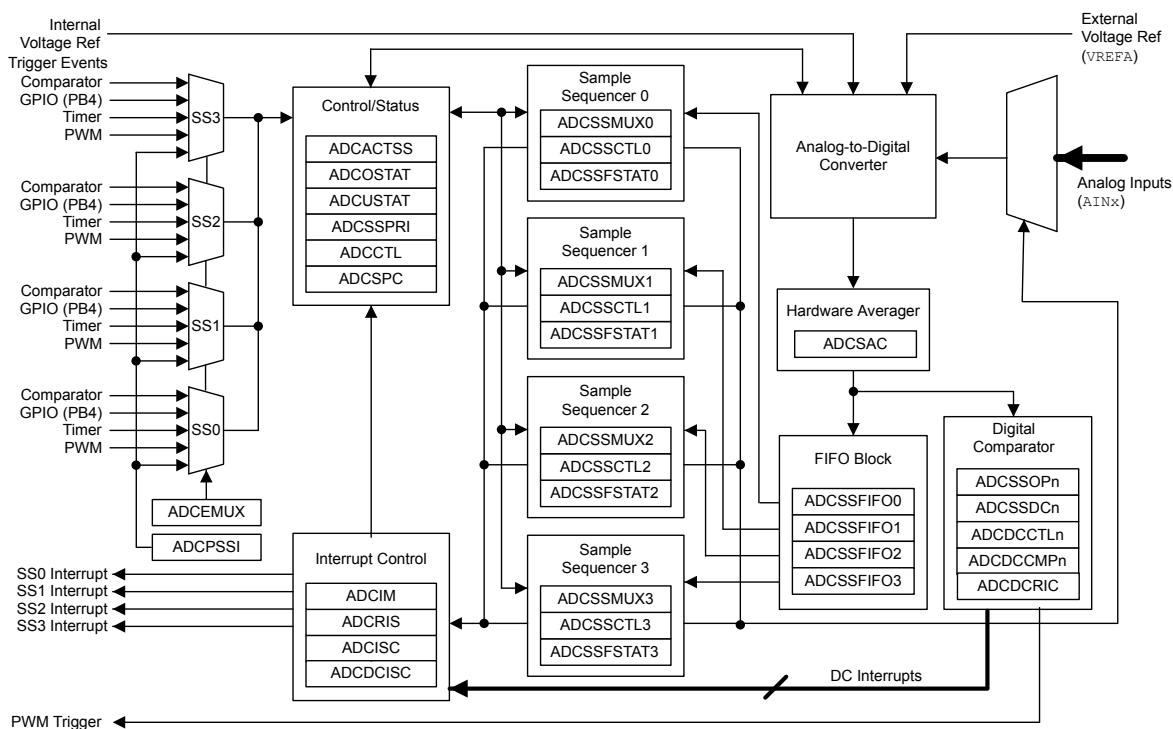
Figure 11-2. ADC Module Block Diagram
