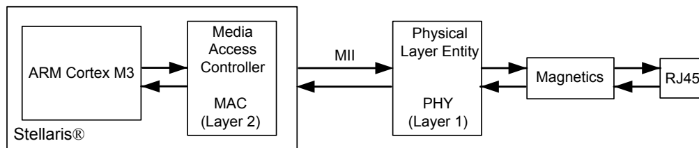
Figure 17-1. Ethernet Controller
