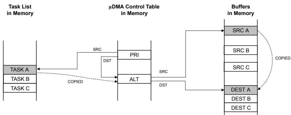
Figure 7-4. Memory Scatter-Gather, \mu DMA Copy Sequence
