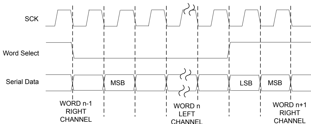
Figure 15-3. Left-Justified Data Transfer
