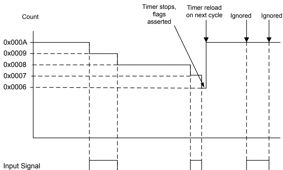
Figure 9-3. Input Edge-Count Mode Example
