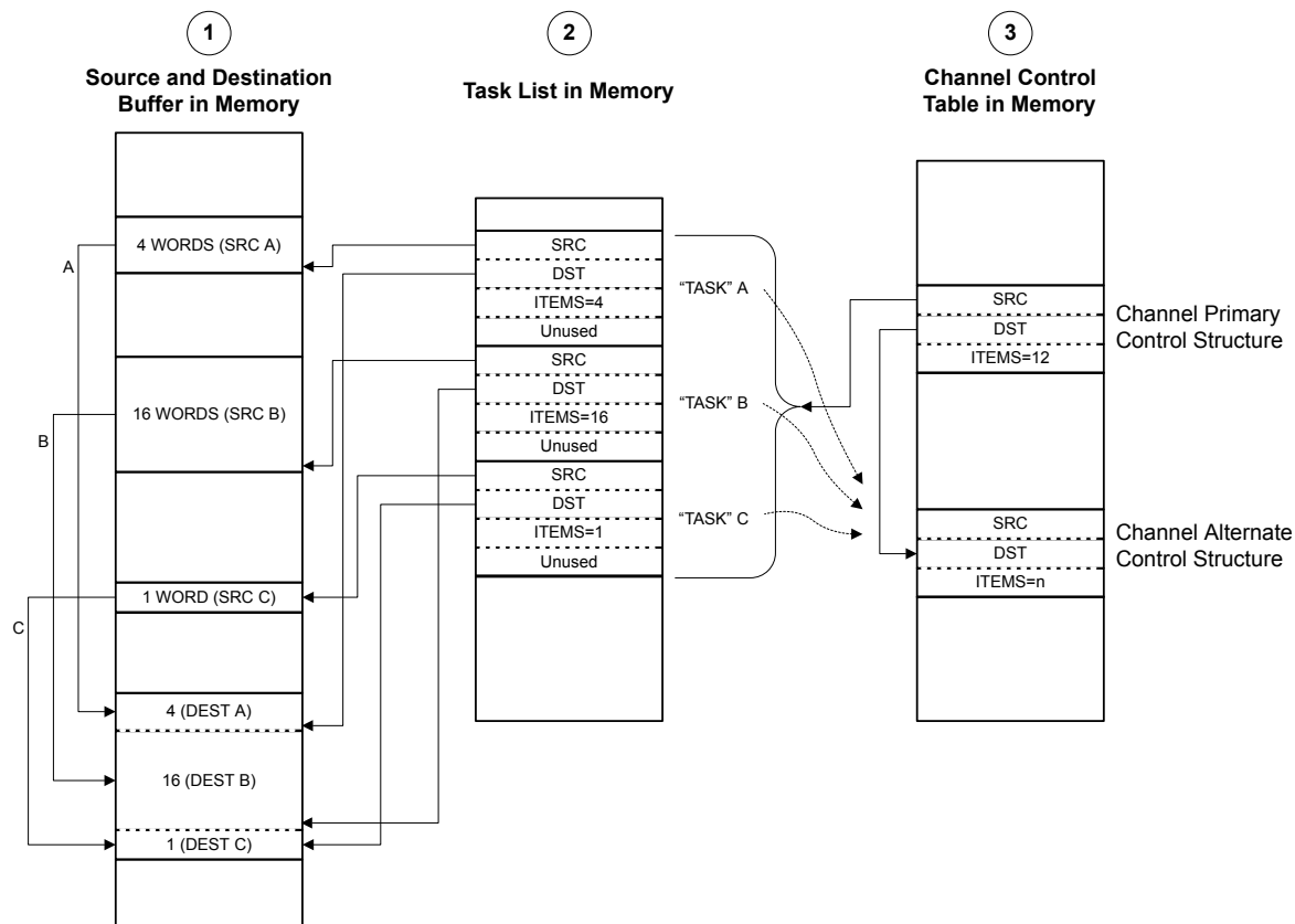
Figure 7-3. Memory Scatter-Gather, Setup and Configuration
