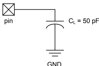
Figure 25-1. Load Conditions
