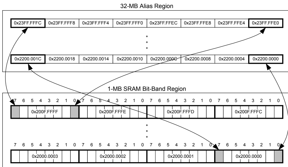
Figure 2-4. Bit-Band Mapping
