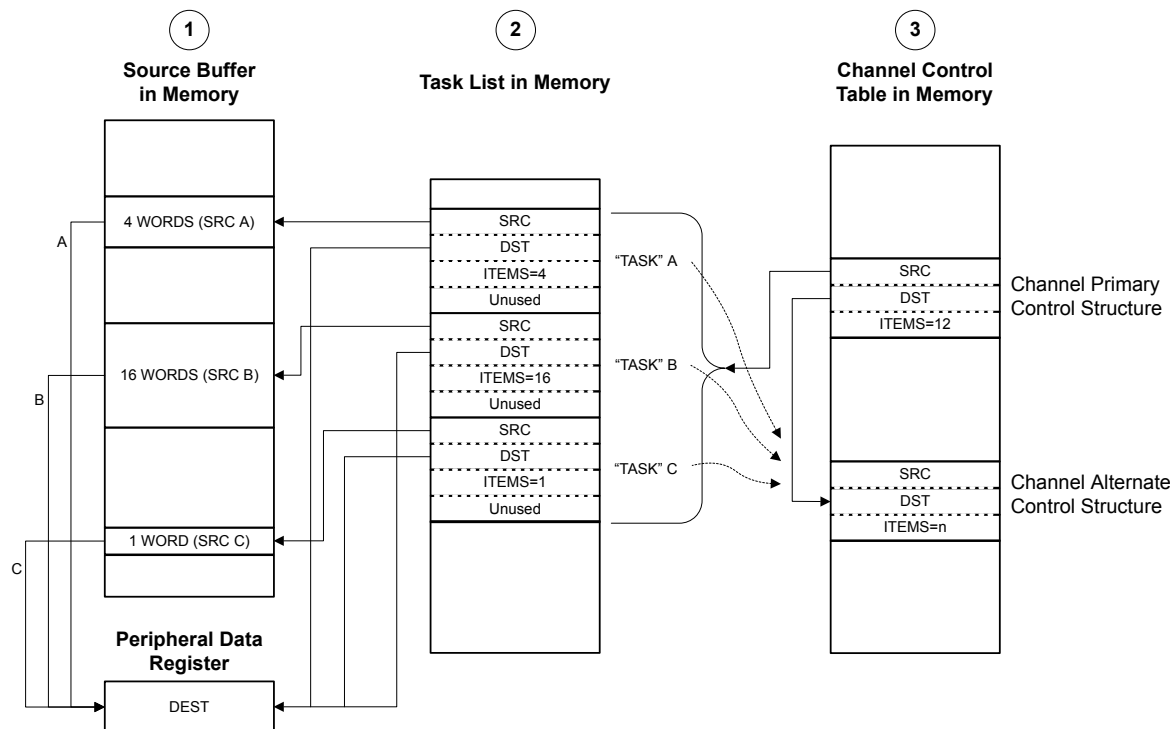
Figure 7-5. Peripheral Scatter-Gather, Setup and Configuration
