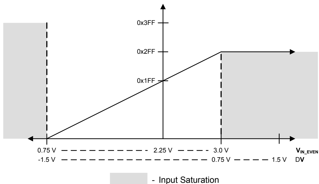
Figure 11-12. Differential Sampling Range, V_{IN\_ODD} = 2.25\text{ V}
