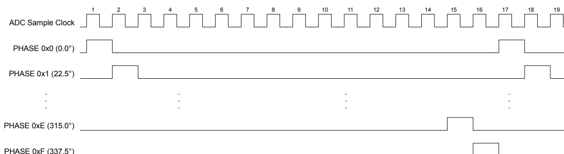
Figure 11-3. ADC Sample Phases
