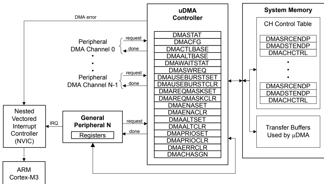
Figure 7-1. \mu DMA Block Diagram
