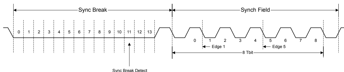
Figure 12-5. LIN Synchronization Field
