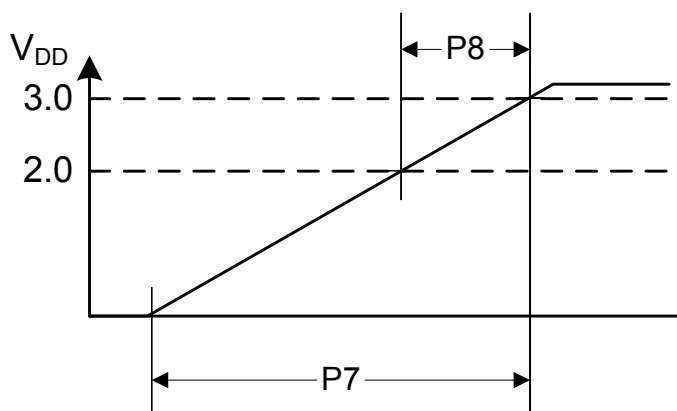
Figure 25-6. Power-On Reset and Voltage Parameters
