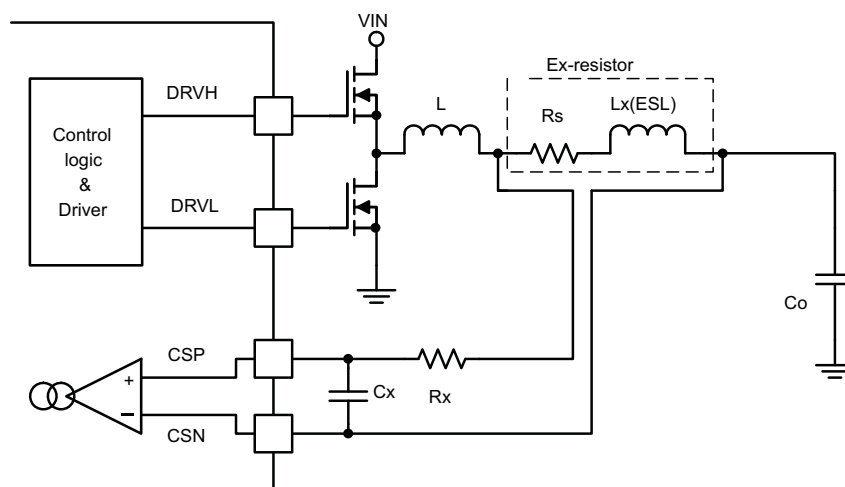
Figure 47. External Resistor Current Sensing
