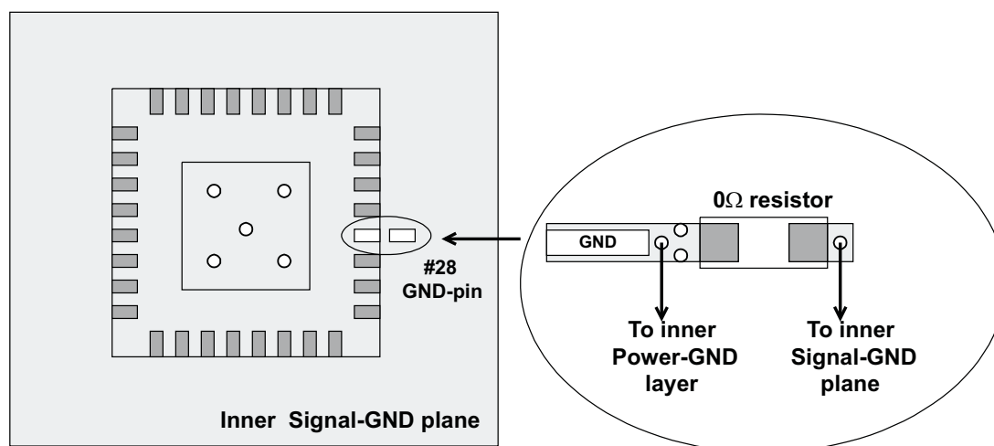
Figure 53. GND Layout Example
