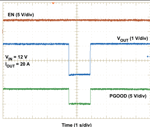
Figure 31. Over-temperature Protection Waveforms
