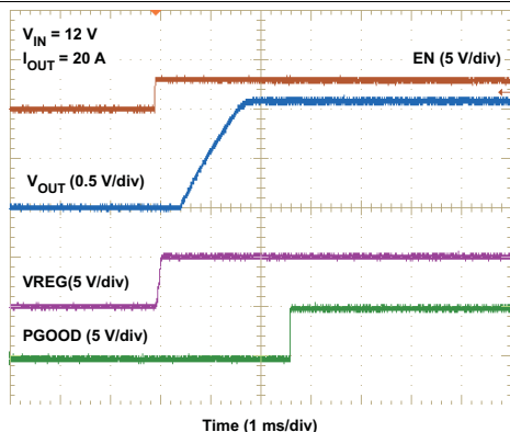
Figure 19. Start-Up Waveforms
