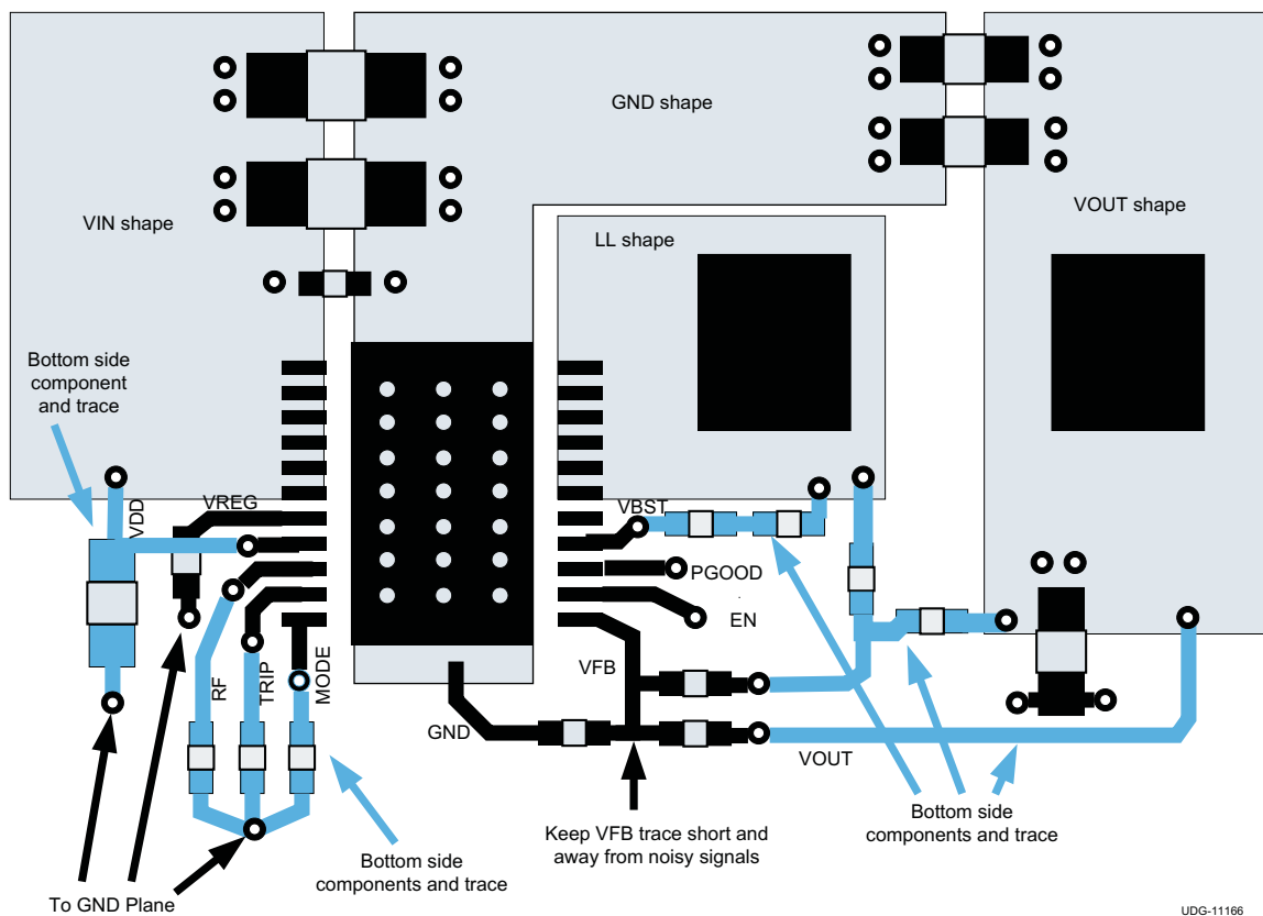
Figure 50. Layout Recommendation
