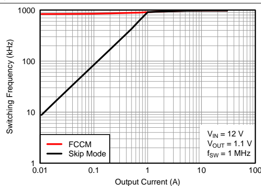
Figure 8. Switching Frequency vs. Output Current
