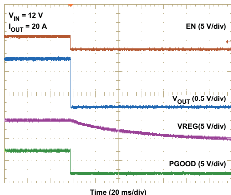
Figure 21. Shutdown Waveforms
