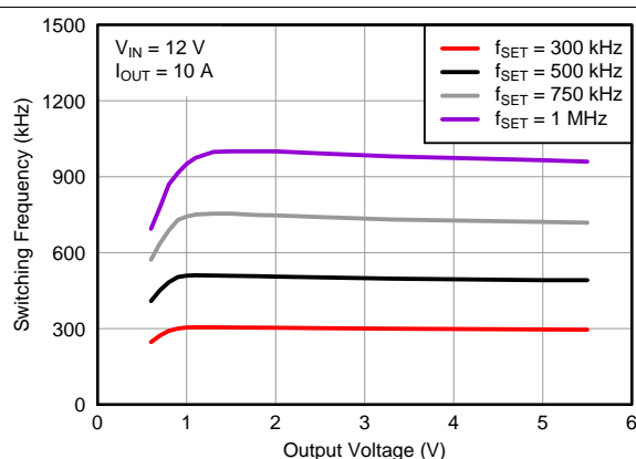
Figure 9. Switching Frequency vs. Output Voltage
