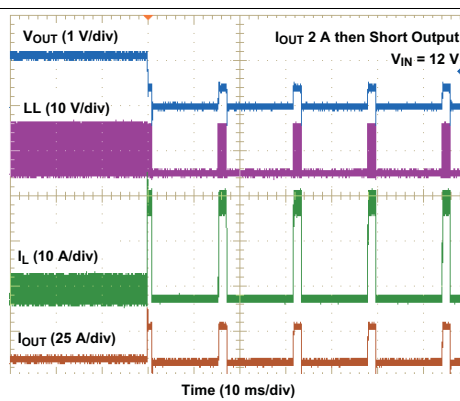
Figure 30. Output Short Circuit Protection Waveforms
