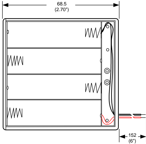
HOLDER
