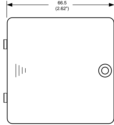
COVER
