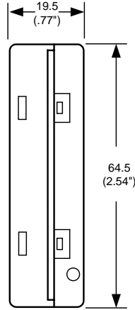
END VIEW
