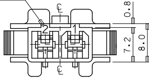
VIEW "A"
