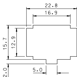
PANEL HOLE DIMENSION
