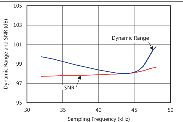
Figure 21. Dynamic Range and SNR vs Sampling Frequency
