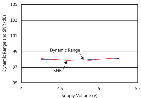
Figure 18. Dynamic Range and SNR vs Supply Voltage
