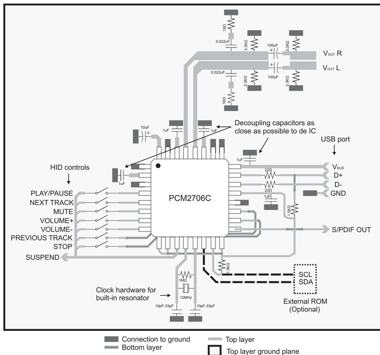
Figure 39. Layout Example 2
