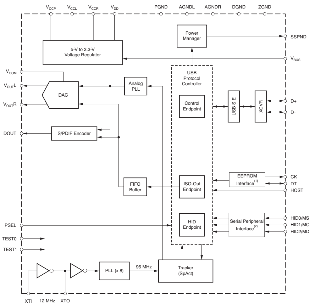
Figure 26. PCM2704C/PCM2705C
