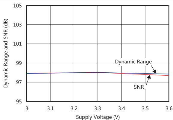
Figure 19. Dynamic Range and SNR vs Supply Voltage
