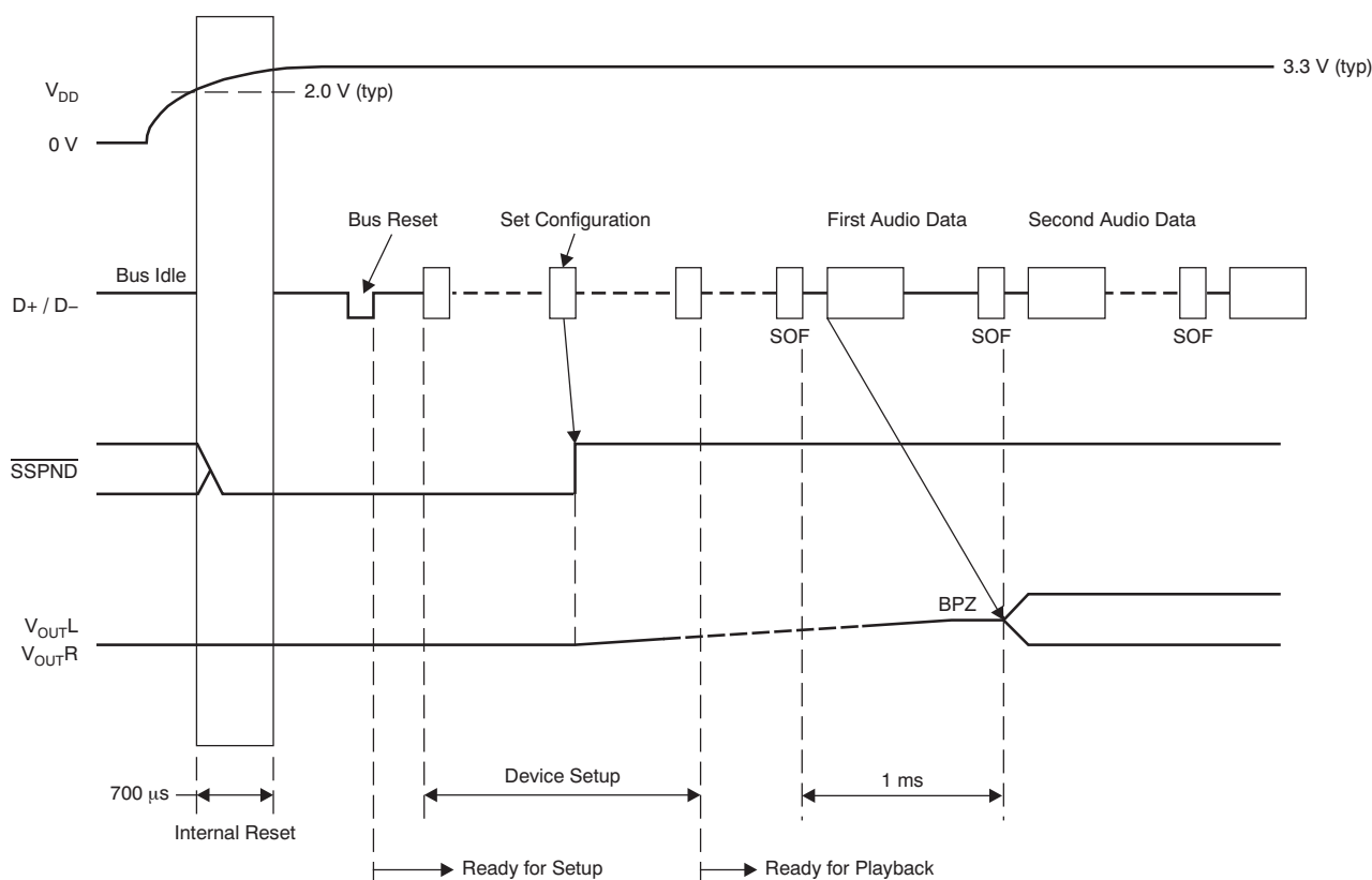
Figure 30. Initial Sequence
