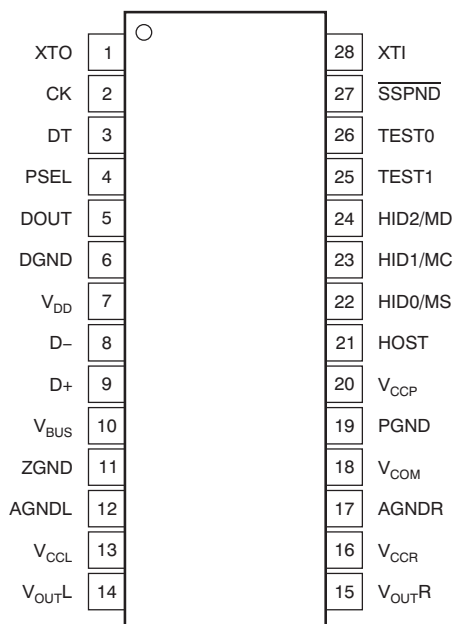
PCM2704C, PCM2705C DB Package 28-Pin SSOP Top View
