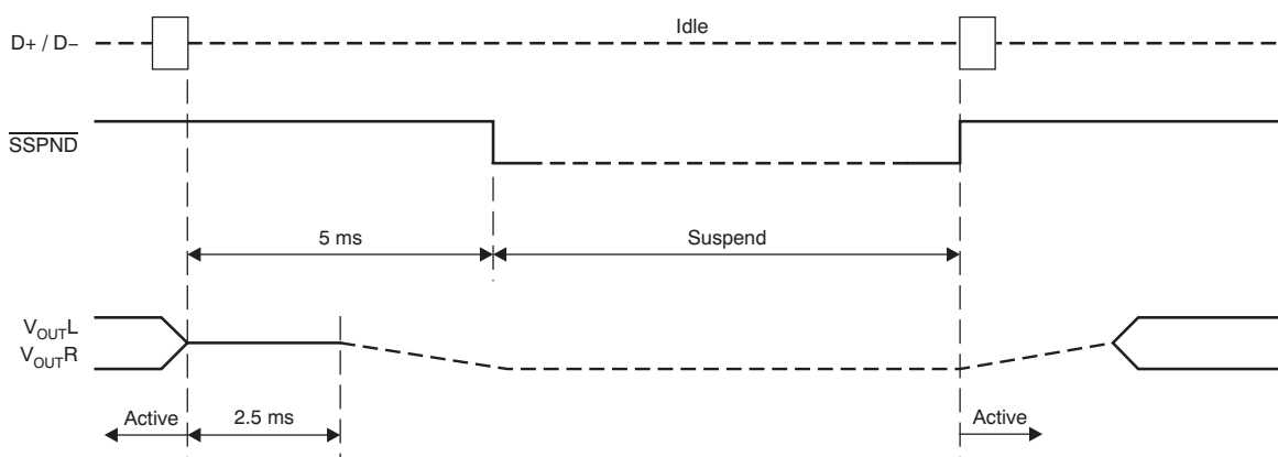
Figure 32. Suspend and Resume
