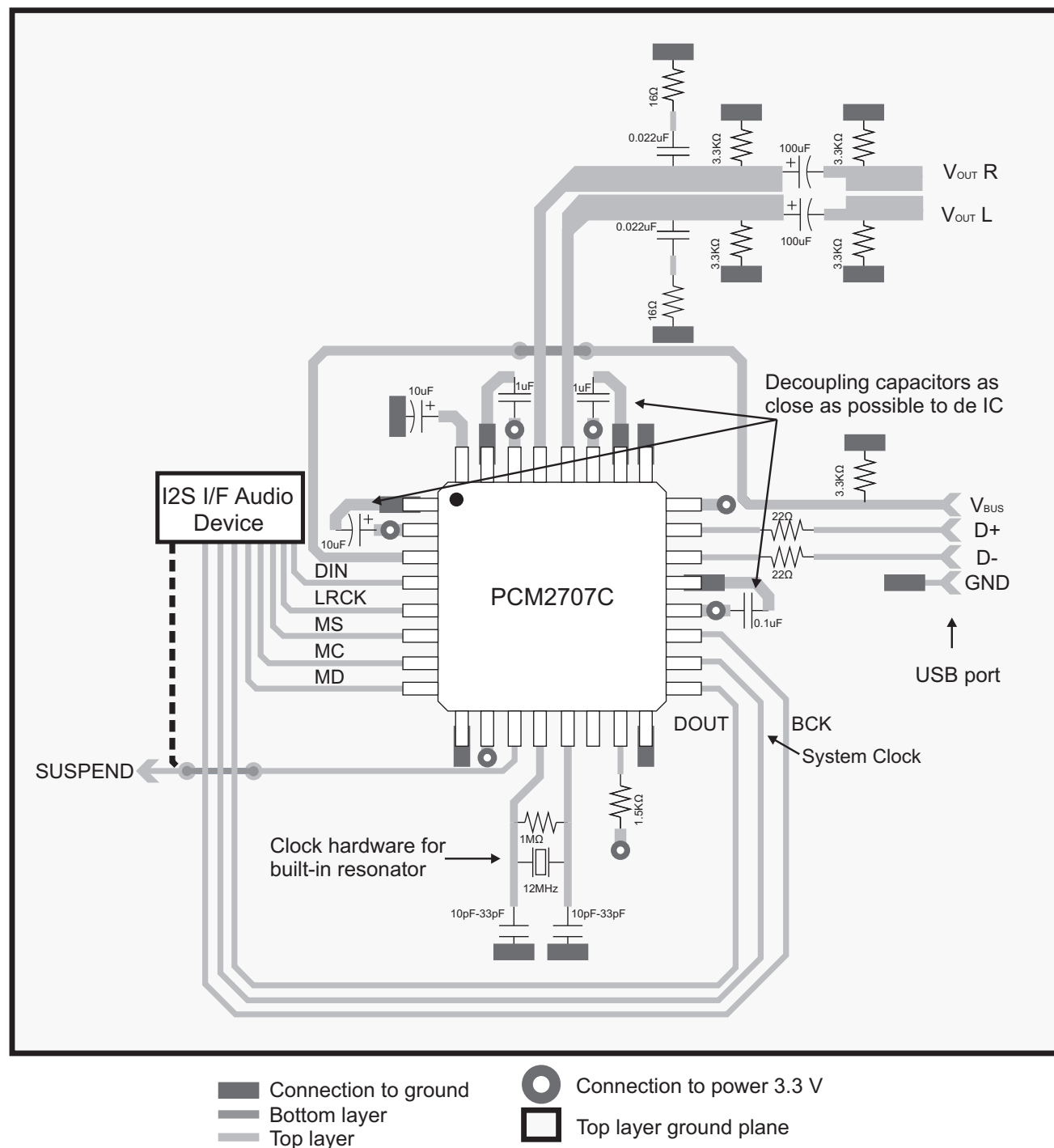
Figure 40. Layout Example 3
