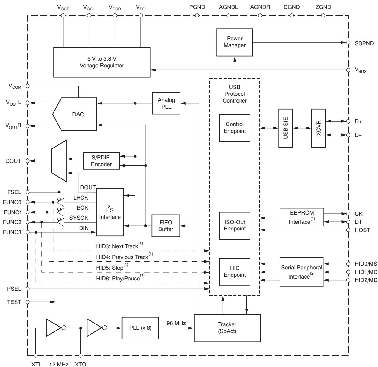
Figure 27. PCM2706C/PCM2707C
