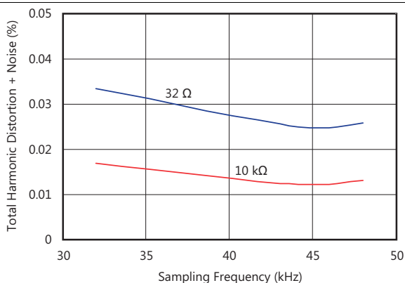
Figure 14. Total Harmonic Distortion + Noise vs Sampling Frequency
