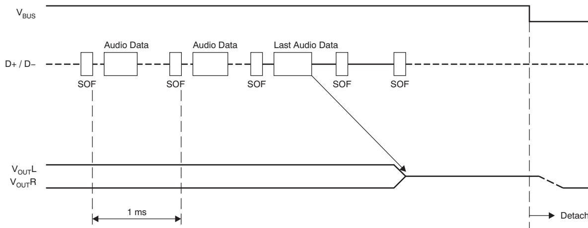
Figure 31. Play, Stop, and Detach Sequence
