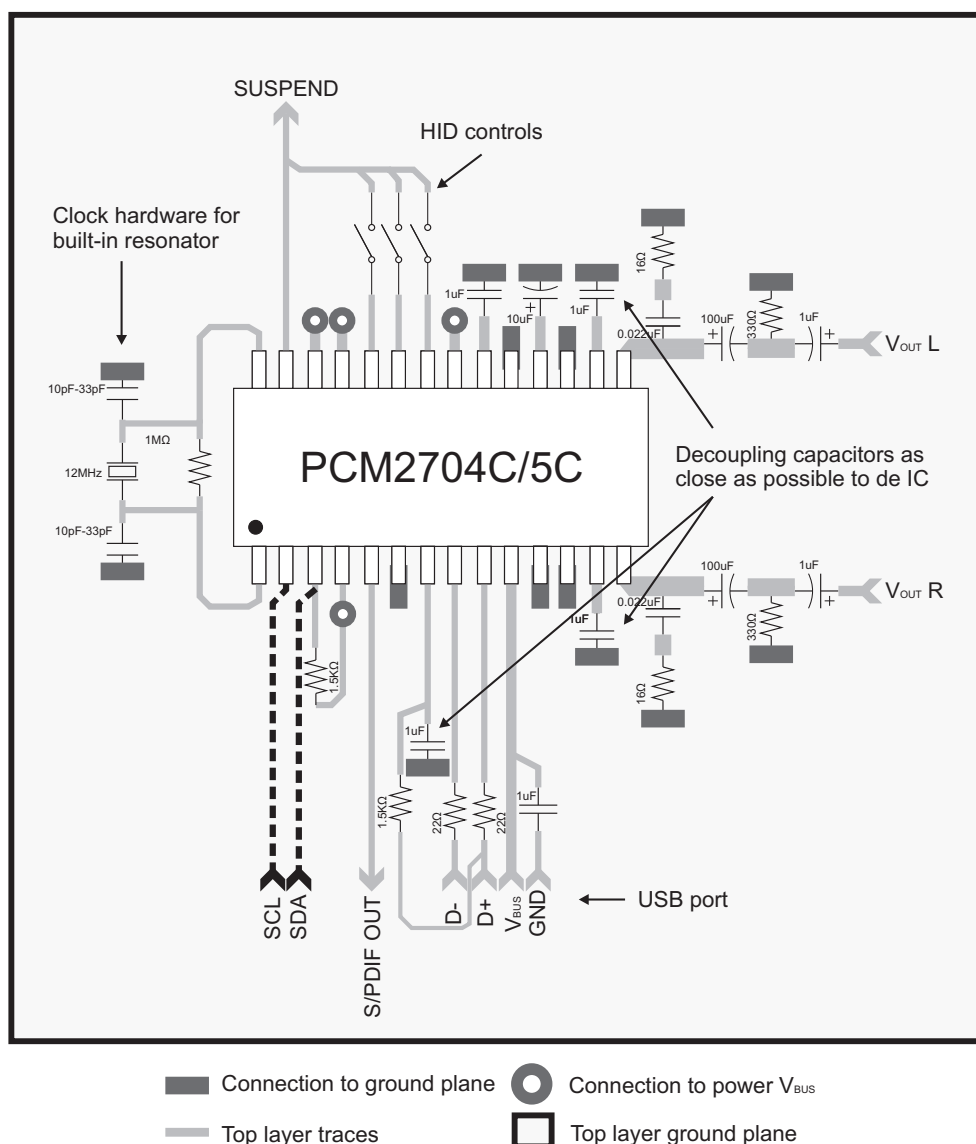
Figure 38. Layout Example 1
