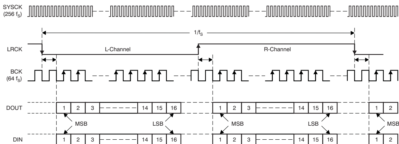
Figure 1. Audio Data Interface Format
