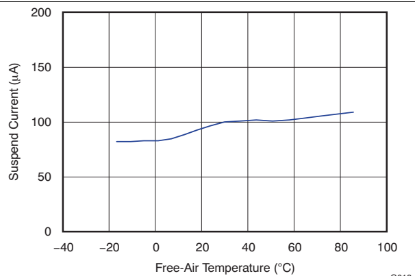
Figure 23. Suspend Current vs Free-Air Temperature
