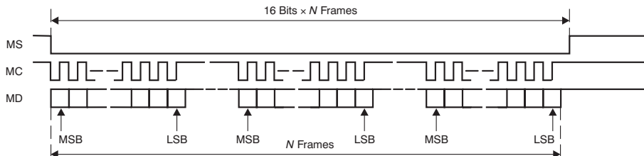
Figure 29. SPI Write Operation
