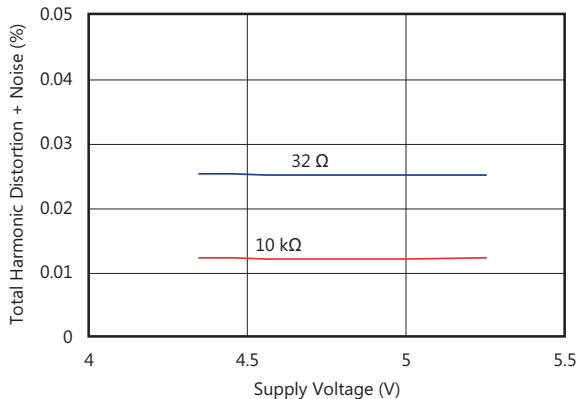
Figure 12. Total Harmonic Distortion + Noise vs Supply Voltage
