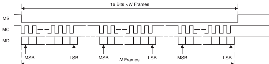
Figure 29. SPI Write Operation
