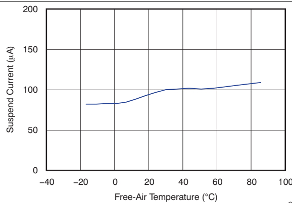
Figure 23. Suspend Current vs Free-Air Temperature
