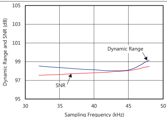
Figure 20. Dynamic Range and SNR vs Sampling Frequency
