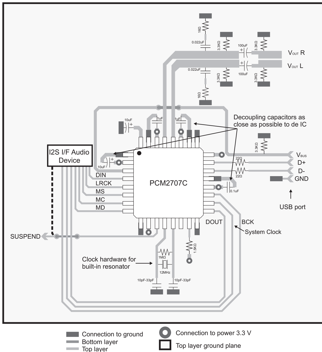
Figure 40. Layout Example 3
