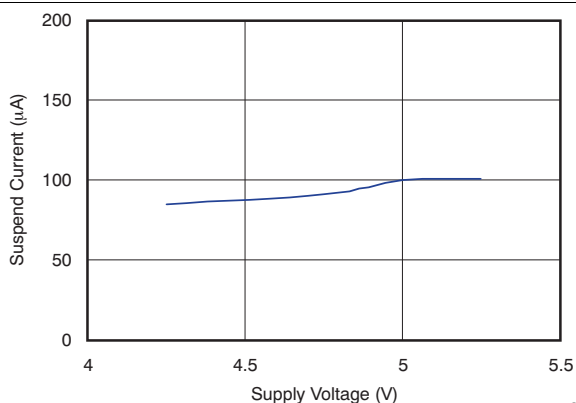
Figure 22. Suspend Current vs Supply Voltage
