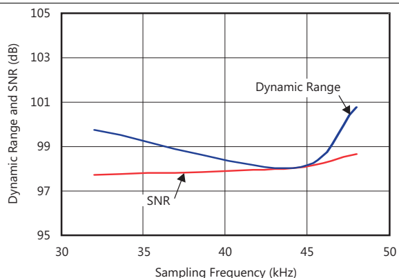
Figure 21. Dynamic Range and SNR vs Sampling Frequency
