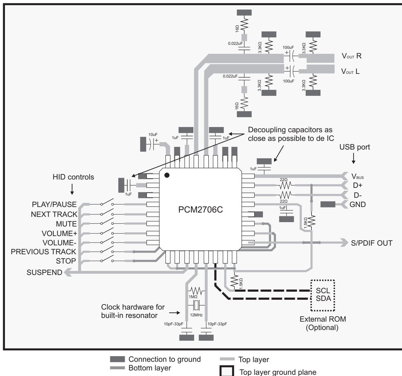
Figure 39. Layout Example 2
