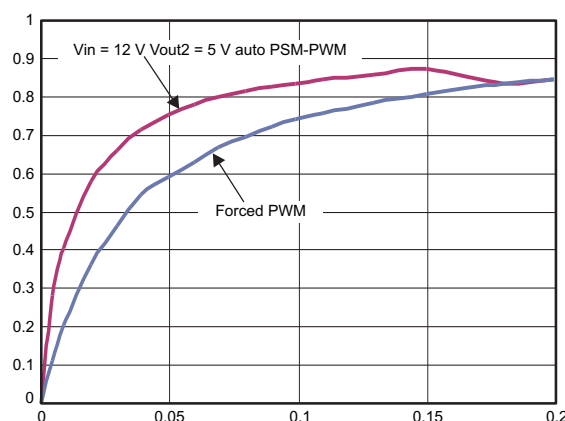
Figure 6. Efficiency Buck 2 at 5 V
