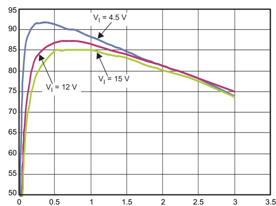
Figure 4. Efficiency Buck 2 at 1 V
