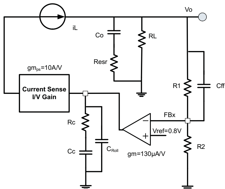
Figure 16. Loop Compensation
