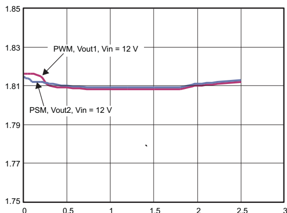
Figure 1. Load Regulation Buck 1 at 1.8 V, 1% Resistors
