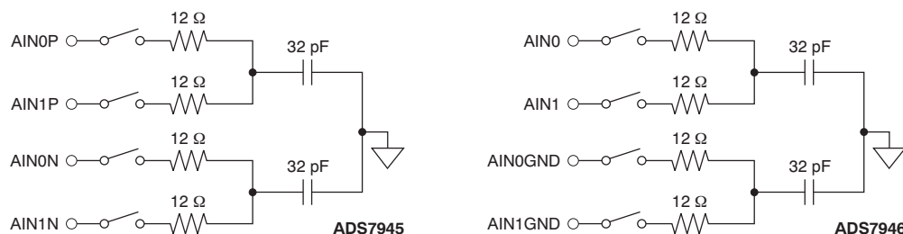
Figure 76. Input Sampling Stage Equivalent Circuit
