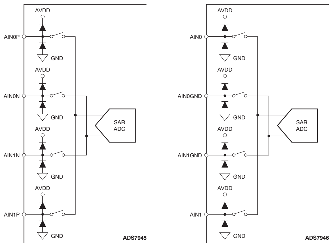
Figure 75. Analog Inputs
