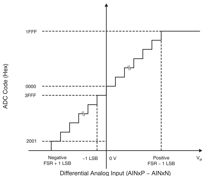
Figure 79. ADS7945 Transfer Characteristics
