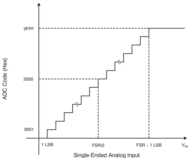
Figure 80. ADS7946 Transfer Characteristics
