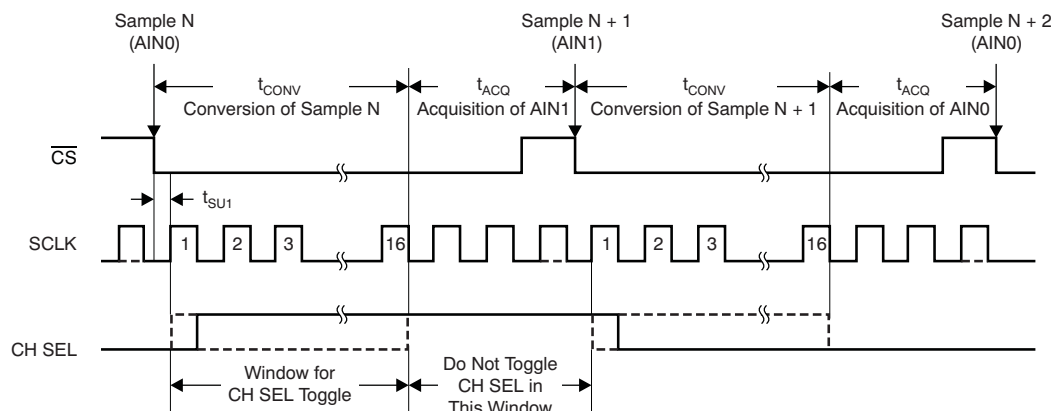
Figure 77. ADC Analog Input Channel Selection
