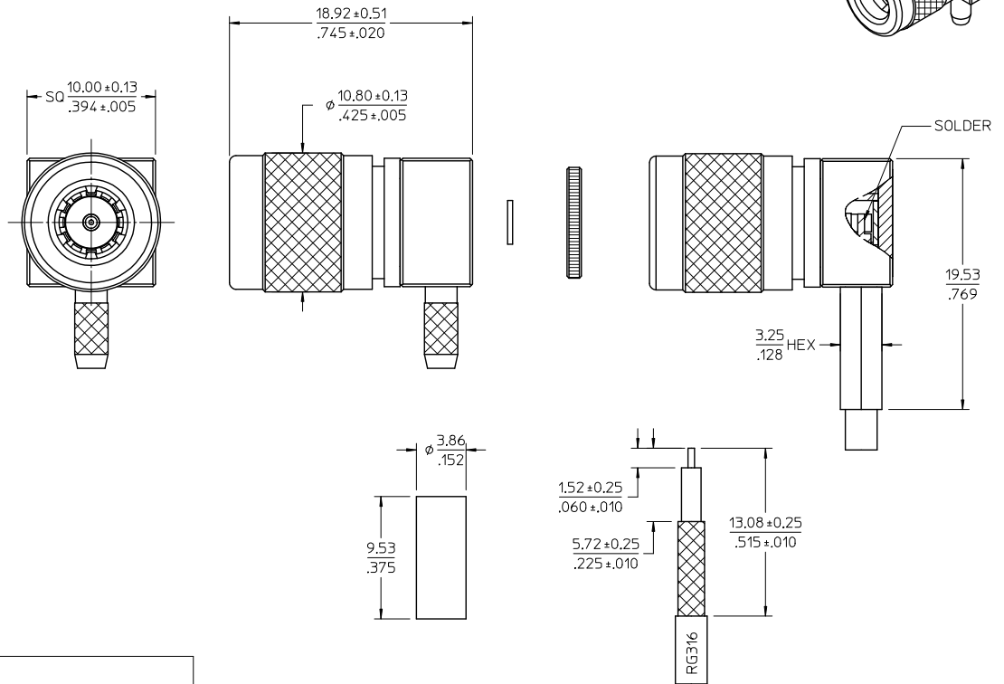
STRIPPING DIMENSIONS
