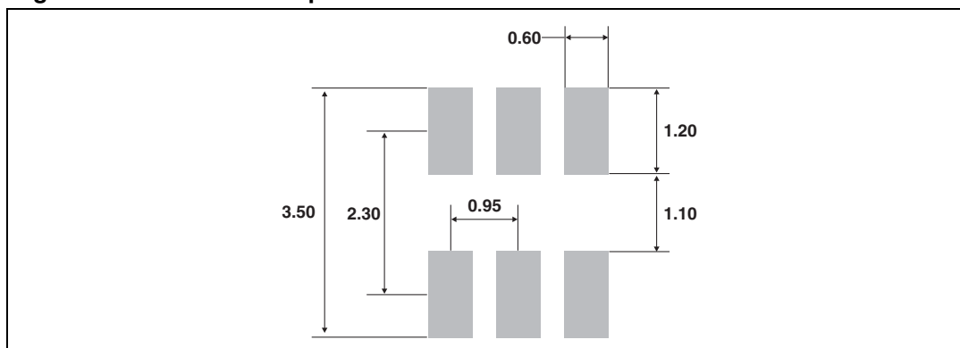
Figure 11. SOT23-6L footprint
